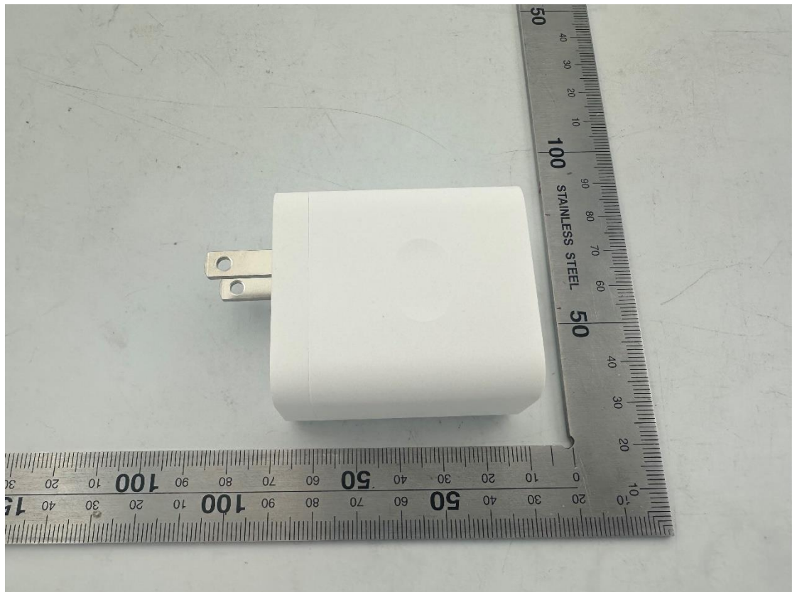
Photo 11 Appearance of adapter (3#: VCB4HAUH)
