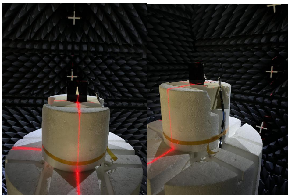
Fig.3. The DUT in the fully anechoic
