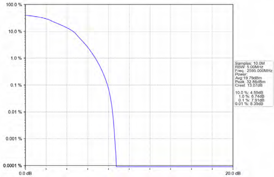
Band38 5MHz 16QAM MCH 2595MHz RB 25 0 NTV
