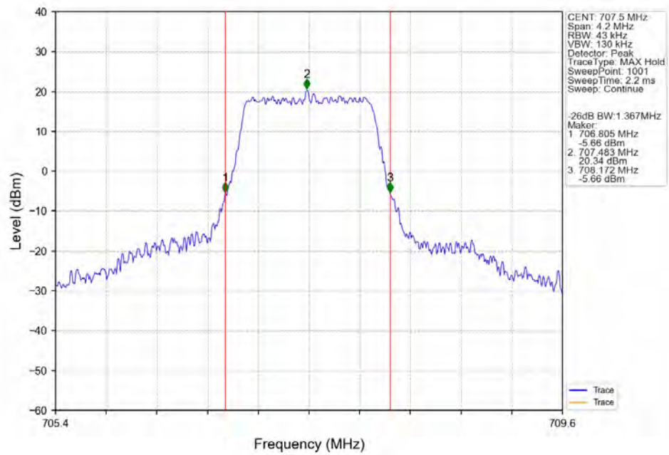
Band12_1.4MHz_QPSK_MCH_707.5MHz_RB_6_0_NTNV
