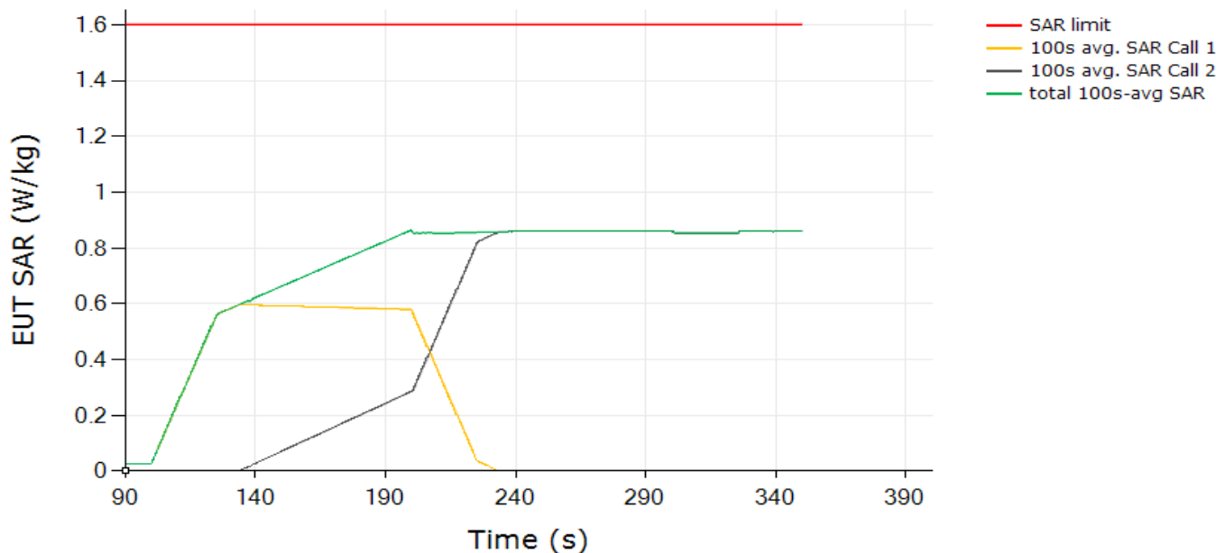
SAR Call Drop Tech: LTE, Band 41
