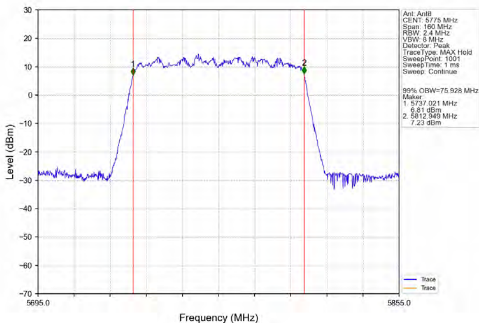
802.11ac(VHT80)_MCH_5775MHz_Ant8_NTNV
