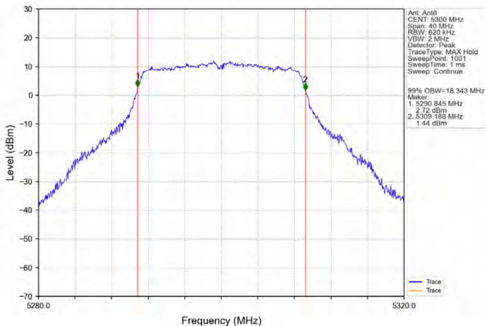
802.11ac(VHT20)_MCH_5300MHz_Ant8_NTNV
