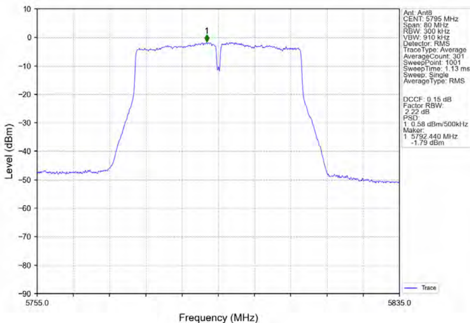
802.11n(HT40)_HCH_5795MHz_Ant8_NTNV
