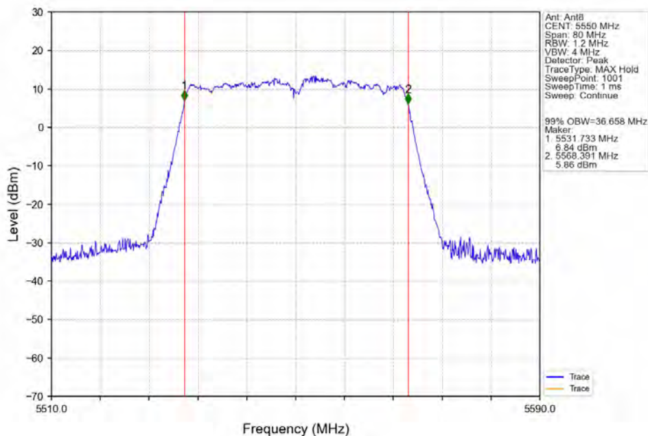
802.11n(HT40)_MCH_5550MHz_Ant8_NTNV
