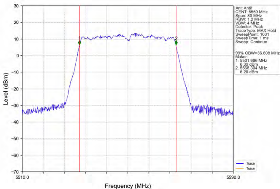
802.11ac(VHT40)_MCH_5550MHz_Ant8_NTNV
