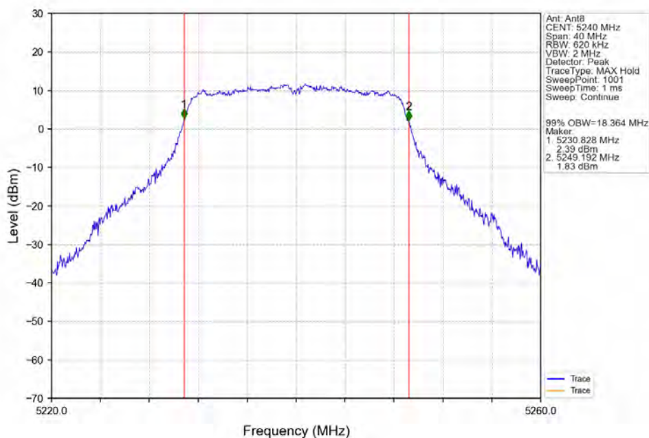
802.11n(HT20)_HCH_5240MHz_Ant8_NTNV
