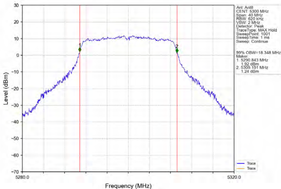
802.11n(HT20)_MCH_5300MHz_Ant8_NTNV
