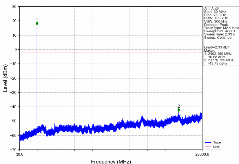
GFSK_DH5_LCH_2402MHz_Ant8_NTNV
