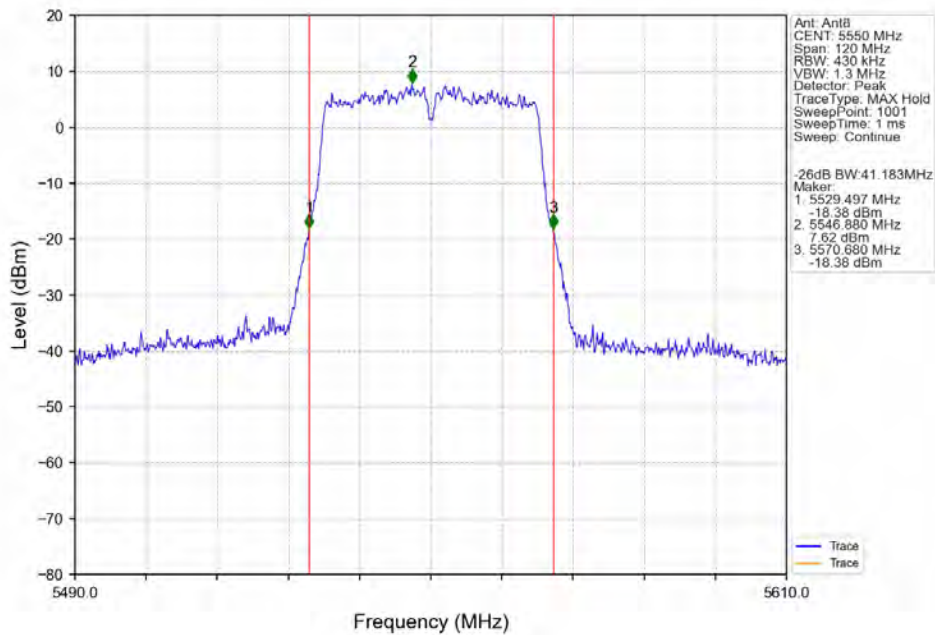
802.11n(HT40) MCH 5550MHz Ant8 NTN
