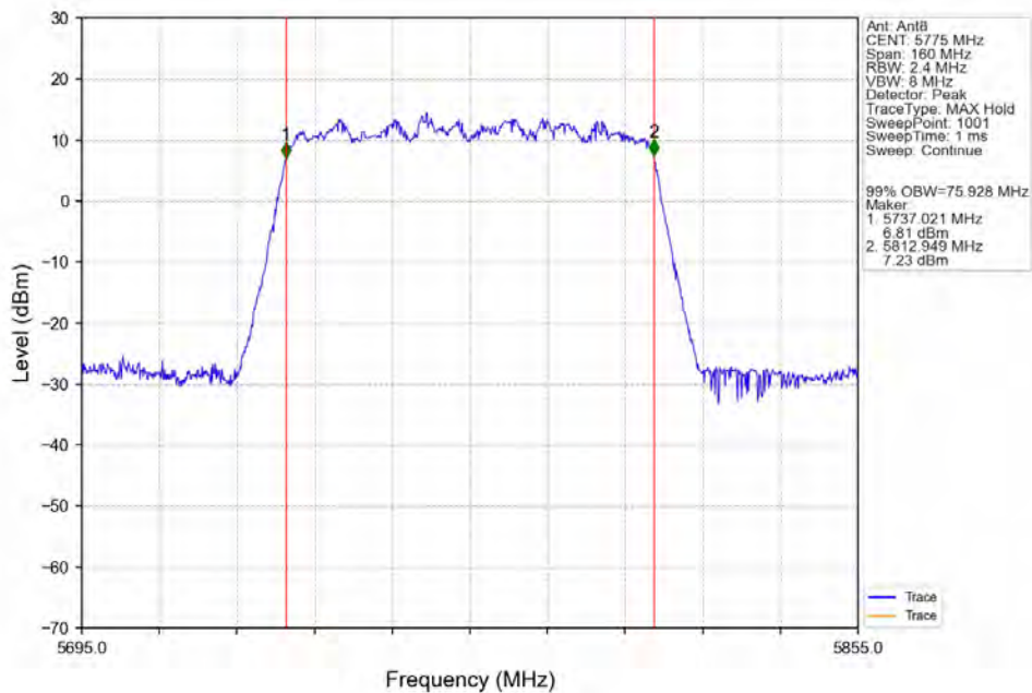
802.11ac(VHT80)_MCH_5775MHz_Ant8_NTNV
