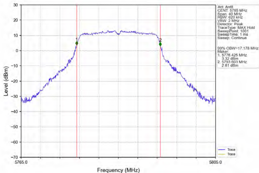
802.11a_MCH_5785MHz_Ant8_NTNV
