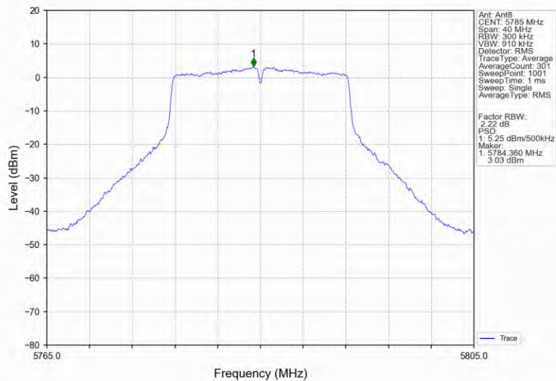
802.11a_MCH_5785MHz_Ant8_NTNV
