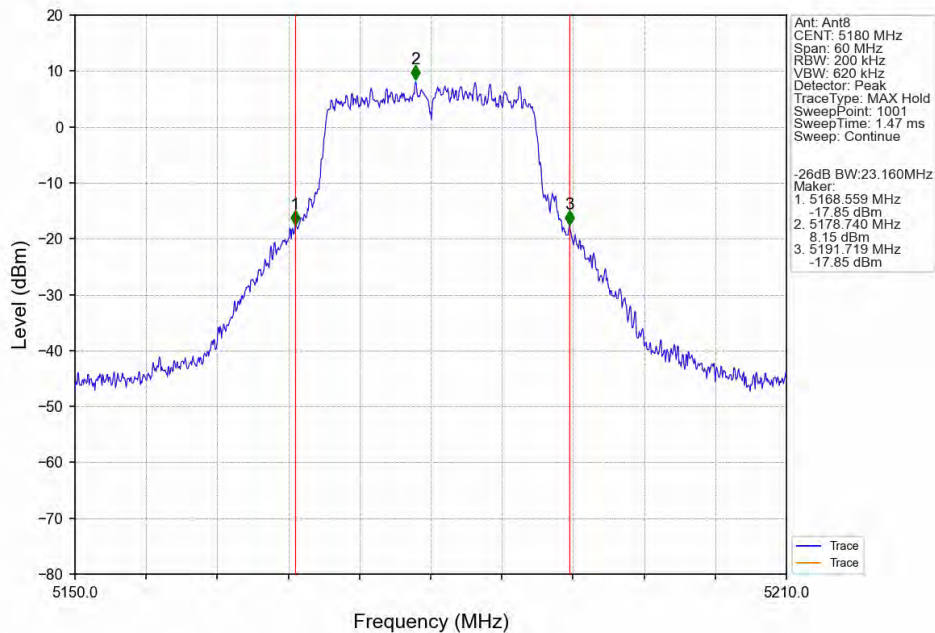
802.11ac(VHT20)_LCH_5180MHz_Ant8_NTNV
