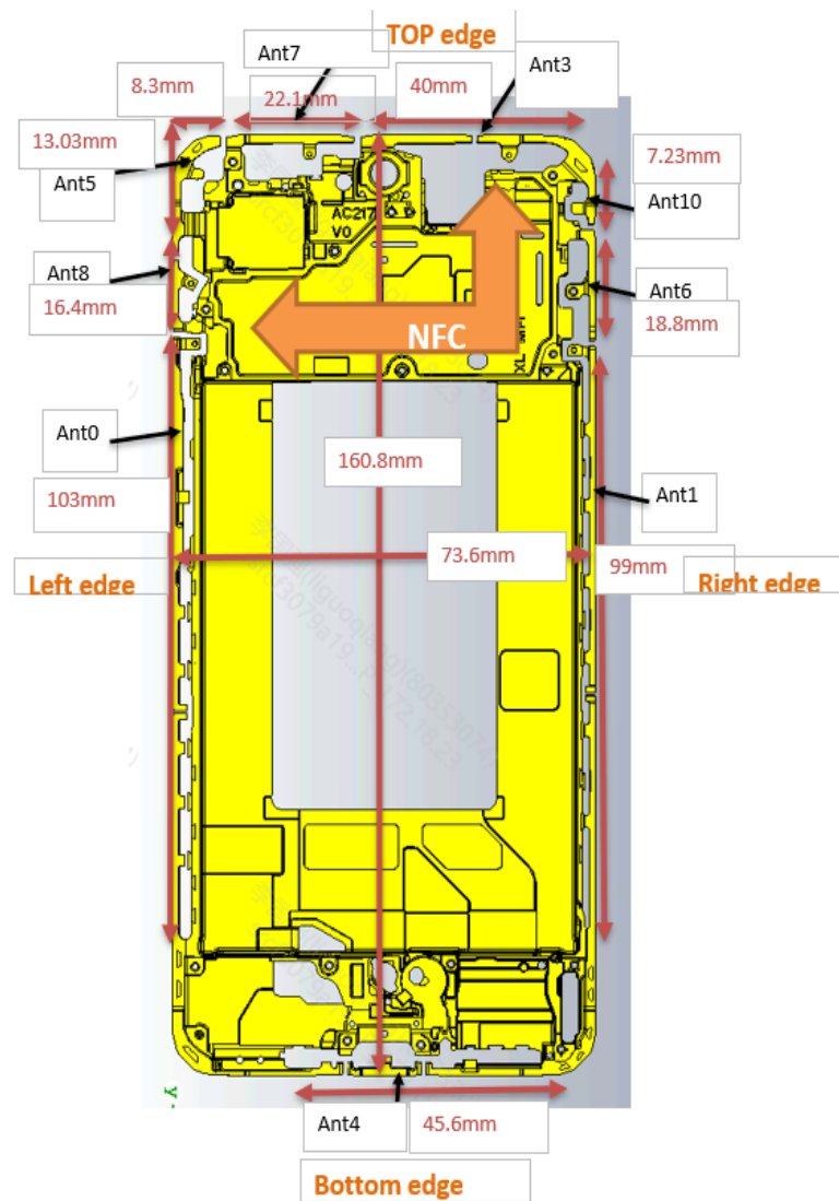
Fig 1 Antenna location&dimension
