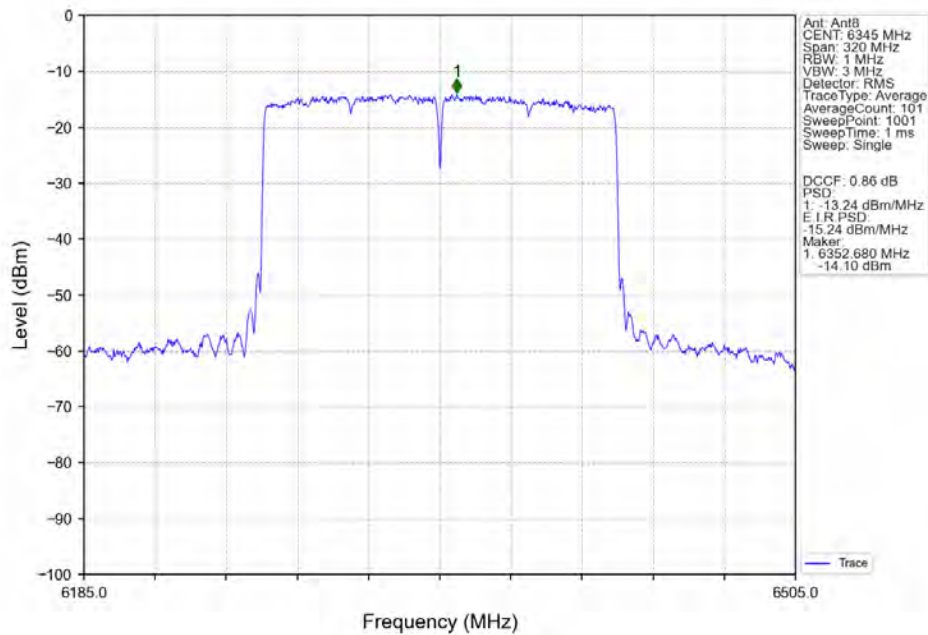
802.11ax(HEW160)_HCH_6345MHz_2xRU996 Left Ant8 NTNV
