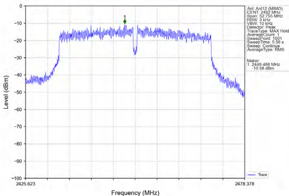
802.11ac(VHT40)_HCH_2452MHz_MIMO_NTNV
