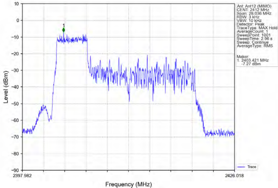
802.11ax(HEW20)_LCH_2412MHz_RU52_Left_MIMO_NTNV
