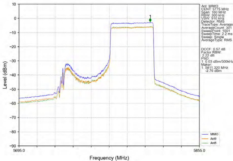
802.11ax(HEW80)_MCH_5775MHz_RU484_Right_MIMO_NTNV
