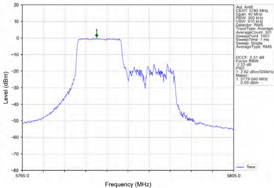
802.11ax(HEW20)_MCH_5785MHz_RU106_Left_Ant8_NTNV
