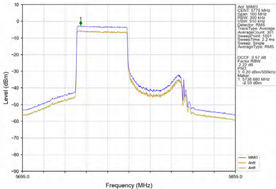
802.11ax(HEW80)_MCH_5775MHz_RU484_Right_Ant9_NTNV
