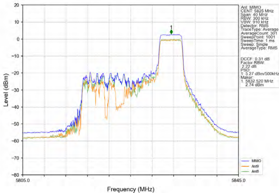
802.11ax(HEW20)_HCH_5825MHz_RU52_Right_MIMO_NTNV
