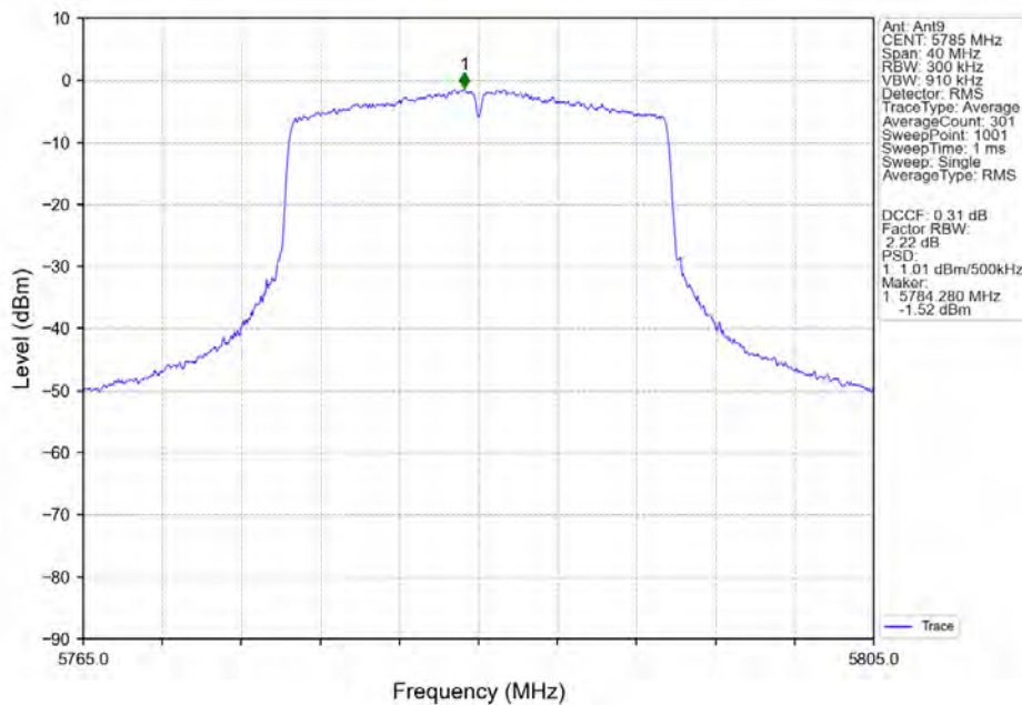
802.11ax(HEW20)_MCH_5785MHz_RU242_Left_Ant9_NTNV
