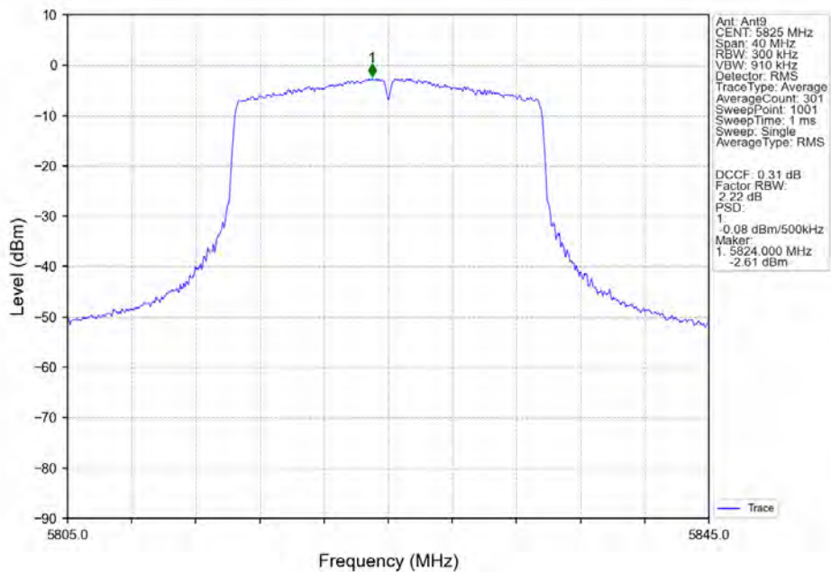
802.11ax(HEW20)_HCH_5825MHz_RU242_Left_Ant9_NTNV
