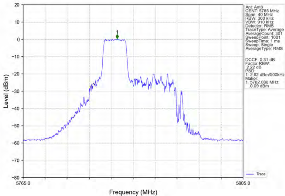
802.11ax(HEW20)_MCH_5785MHz_RU52_Mid_MIMO_NTNV
