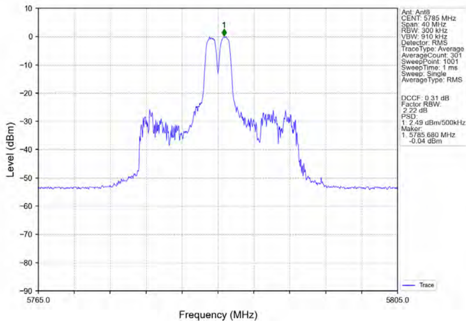
802.11ax(HEW20)_MCH_5785MHz_RU26_Mid_Ant8_NTNV
