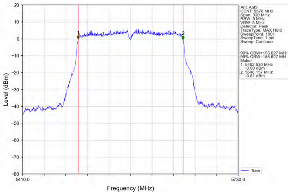
802.11ac(VHT160)_MCH_5570MHz_Ant9_NTNV
