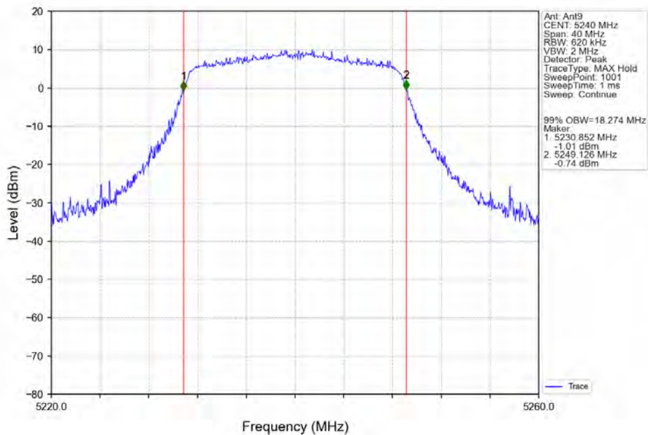
802.11ac(VHT20)_HCH_5240MHz_Ant9_NTNV
