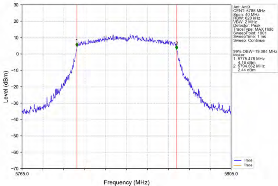
802.11ax(HEW20)_MCH_5785MHz_RU242_Left_Ant9_NTNV
