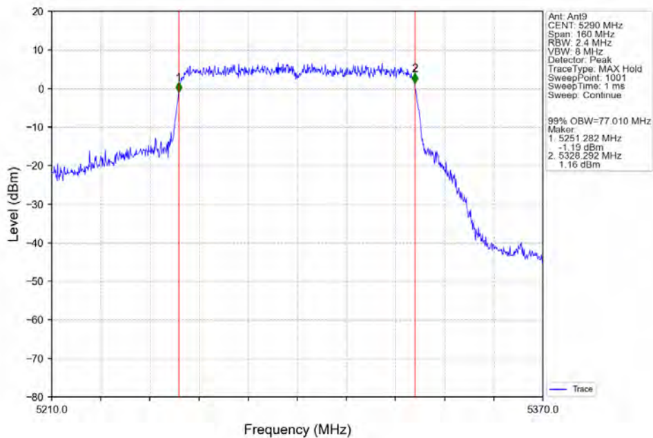
802.11ac(VHT80)_MCH_5290MHz_Ant9_NTNV
