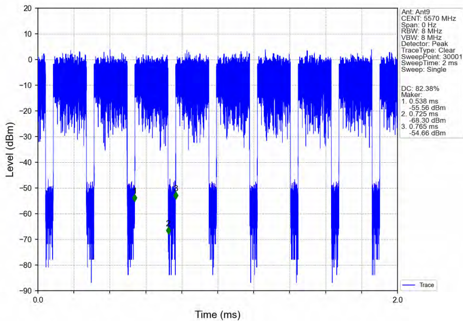
802.11ac(VHT160)_MCH_5570MHz_Ant9_NTNV
