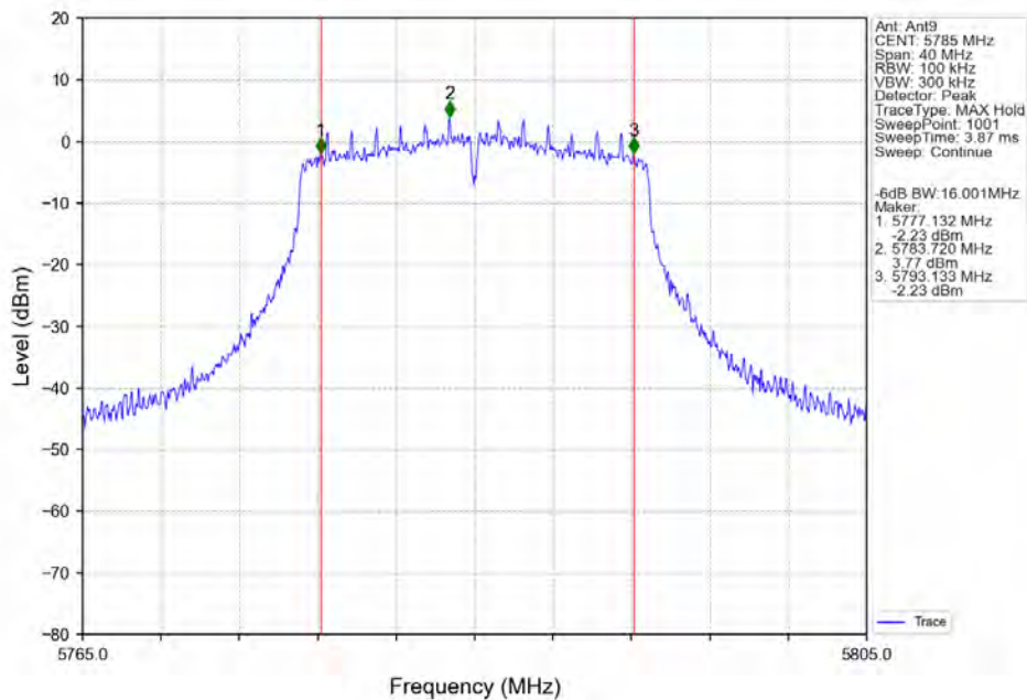
802.11ac(VHT20)_MCH_5785MHz_Ant9_NTNV
