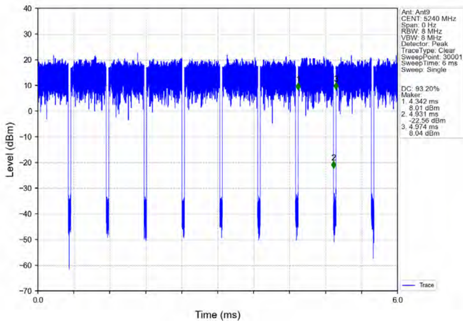
802.11ax(HEW20)_HCH_5240MHz_RU242_Left_Ant9_NTNV
