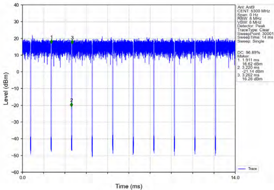
802.11ac(VHT20)_MCH_5300MHz_Ant9_NTNV
