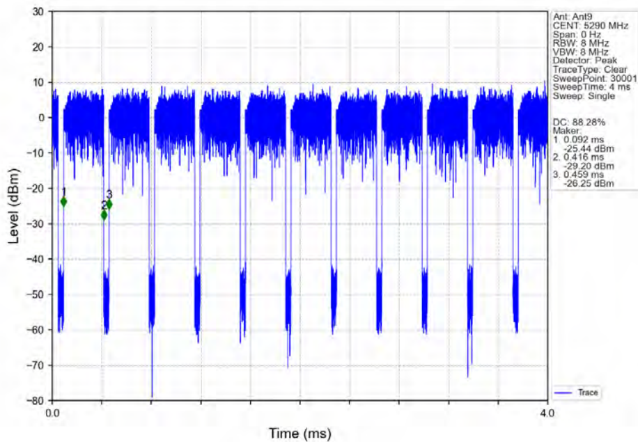
802.11ac(VHT80)_MCH_5290MHz_Ant9_NTNV
