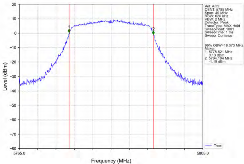
802.11ac(VHT20)_MCH_5785MHz_Ant9_NTNV
