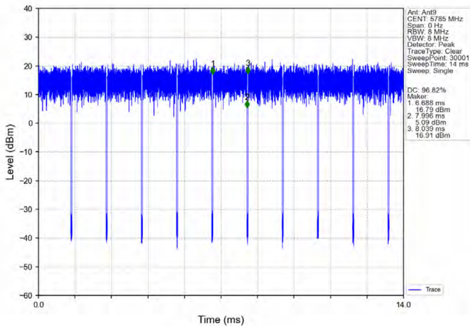
802.11ac(VHT20)_MCH_5785MHz_Ant9_NTNV
