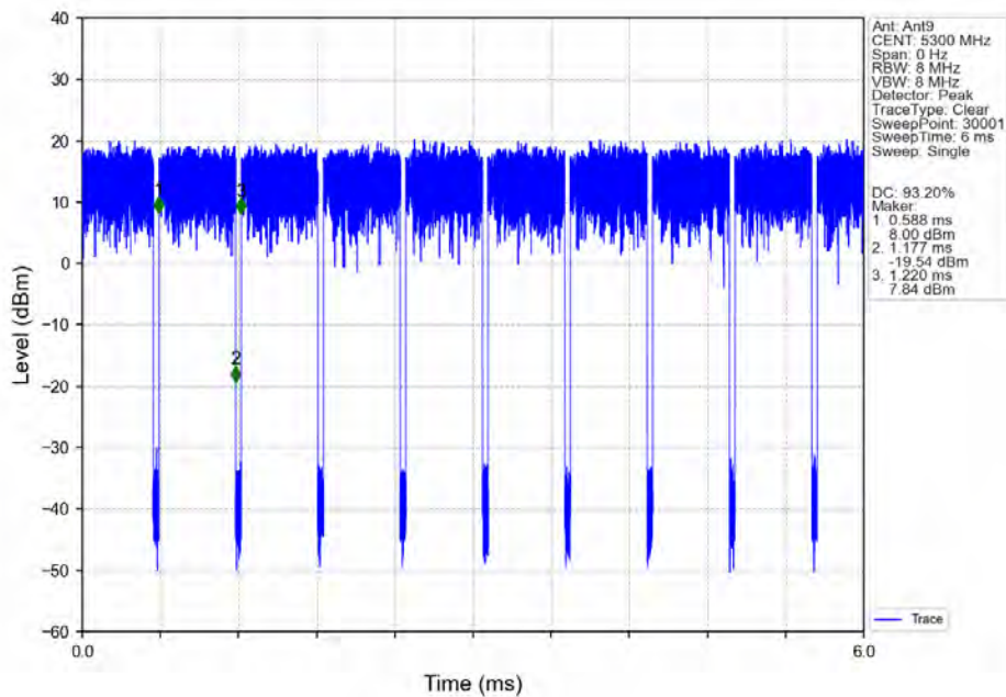
802.11ax(HEW20)_MCH_5300MHz_RU242_Left_Ant9_NTNV
