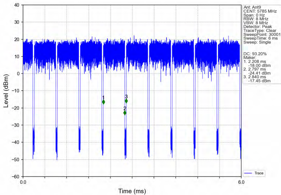
802.11ax(HEW20)_MCH_5785MHz_RU242_Left_Ant9_NTNV
