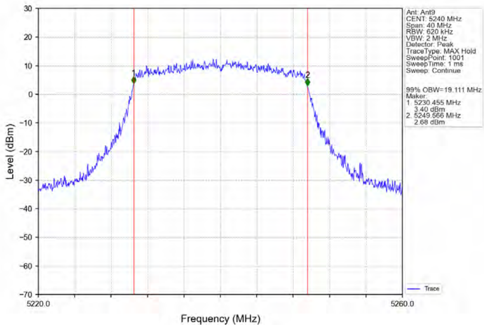
802.11ax(HEW20)_HCH_5240MHz_RU242_Left_Ant9_NTNV
