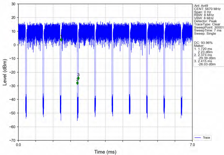
802.11ac(VHT40)_HCH_5670MHz_Ant9_NTNV
