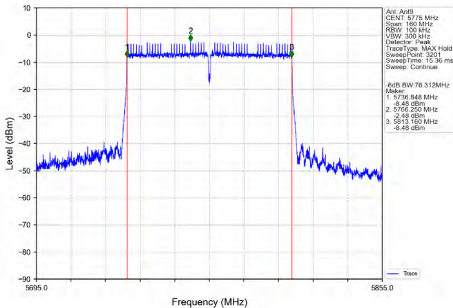
802.11ac(VHT80)_MCH_5775MHz_Ant9_NTNV
