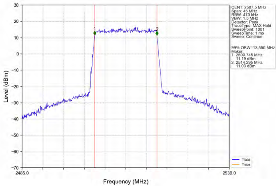
Band7_15MHz_256QAM_LCH_2507.5MHz_RB_75_0_NTN
