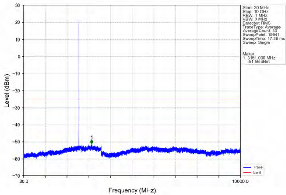
Band7_5MHz_256QAM_HCH_2567.5MHz_RB_1_0_NTNV
