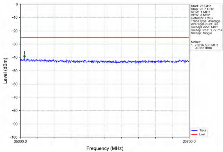
Band7_5MHz_64QAM_LCH_2502.5MHz_RB_1_0_NTV
