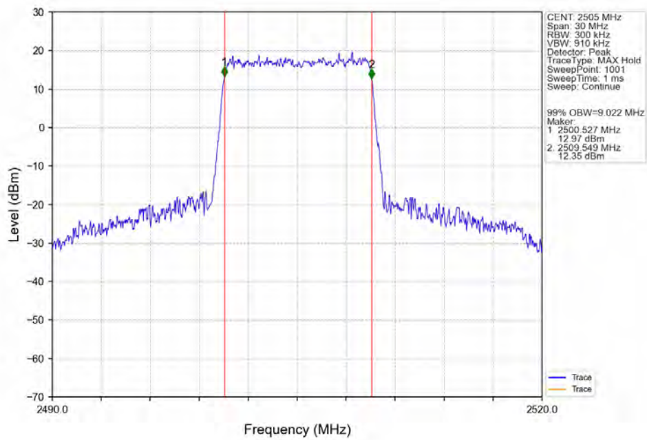
Band7_10MHz_16QAM_LCH_2505MHz_RB_50_0_NTV
