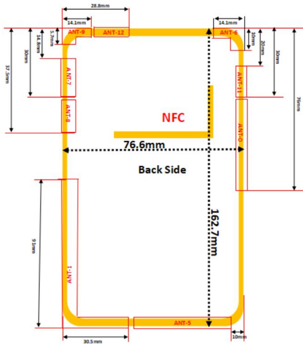
Fig 1 Antenna location&dimension
