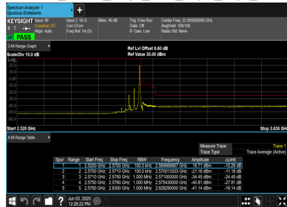
N7(5M)_DFT-s- OFDM_QPSK_Edge_1RB_Right_High_CH
