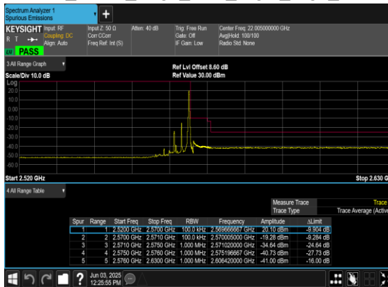
N7(5M)_DFT-s- OFDM_BPSK_Edge_1RB_Right_High_CH
