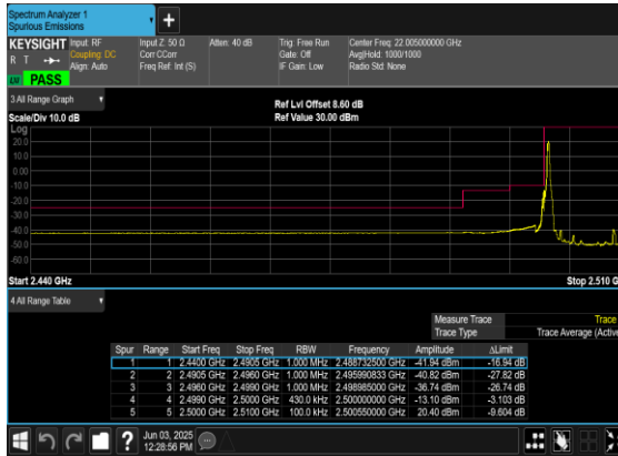
N7(20M)_DFT-s- OFDM_BPSK_Edge_1RB_Left_Low_CH
