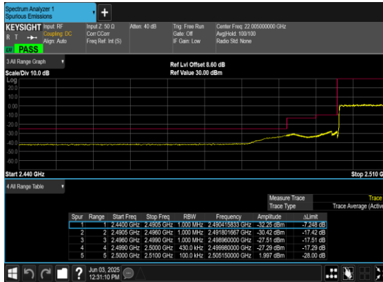
N7(20M)_DFT-s- OFDM_BPSK_Outer_Full_Low_CH
