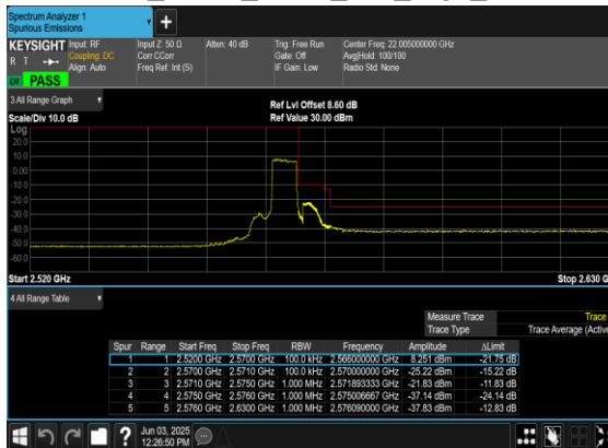
N7(5M)_DFT-s- OFDM_BPSK_Outer_Full_High_CH
