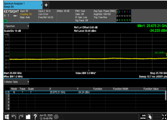
N7(40M)_DFT-s- OFDM_QPSK_Edge_1RB_Left_Mid_CH
