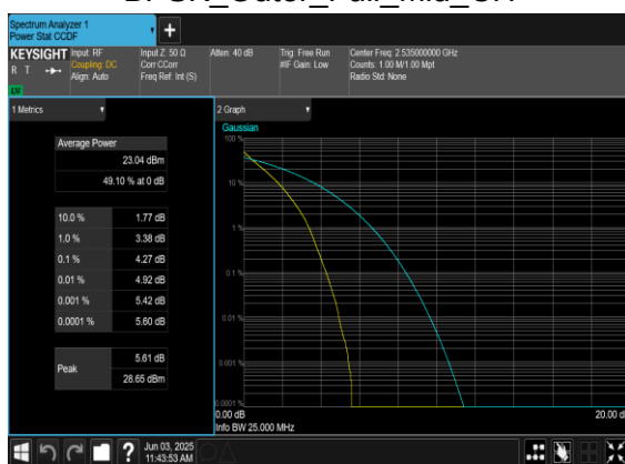
N7(20M)_DFT-s-OFDM_PI_2-BPSK_Outer_Full_Mid_CH
