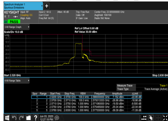
N7(5M)_DFT-s- OFDM_QPSK_Outer_Full_High_CH
