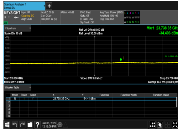
N7(20M)_DFT-s- OFDM_BPSK_Edge_1RB_Left_High_CH
