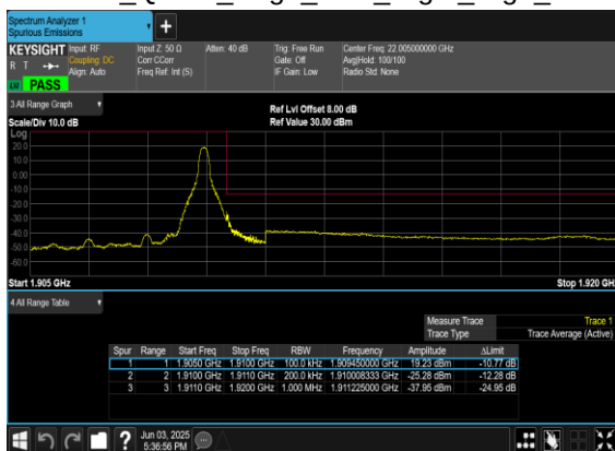
N2(20M)_DFT-s- OFDM_QPSK_Edge_1RB_Right_High_CH
