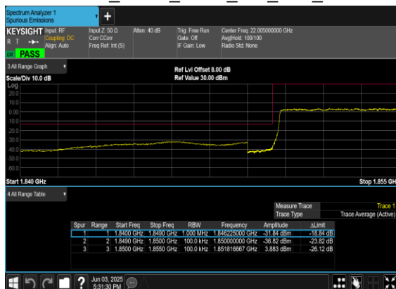
N2(10M)_DFT-s- OFDM_BPSK_Outer_Full_Low_CH
