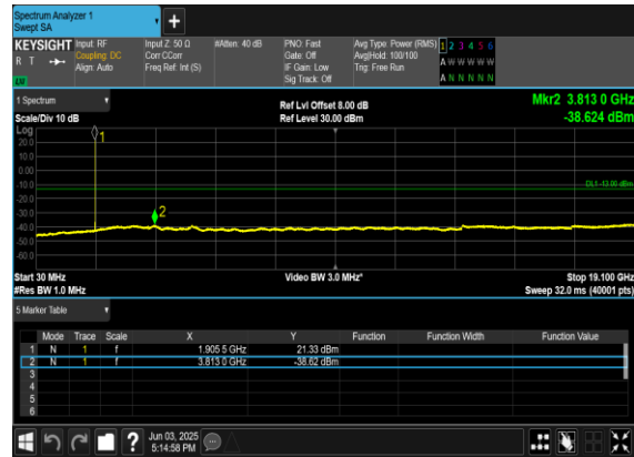
N2(5M)_DFT-s- OFDM_QPSK_Edge_1RB_Left_High_CH
