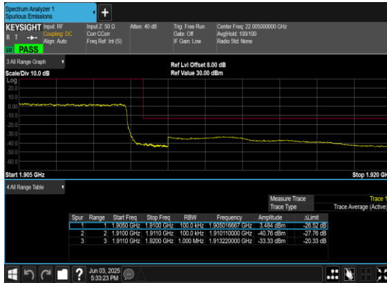
N2(10M)_DFT-s- OFDM_BPSK_Outer_Full_High_CH
