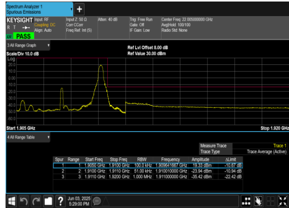
N2(5M)_DFT-s- OFDM_QPSK_Edge_1RB_Right_High_CH
