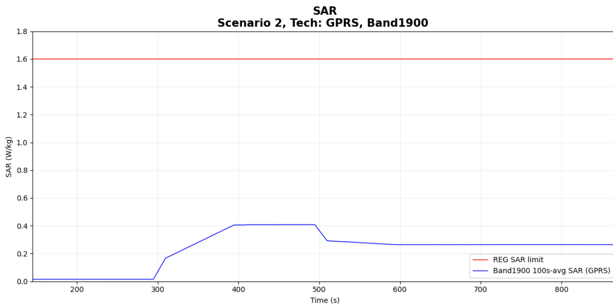
Figure 7-4 Time-averaged SAR
