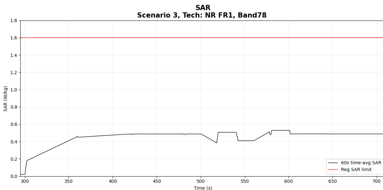
Figure 6- 21 Time-averaged SAR
