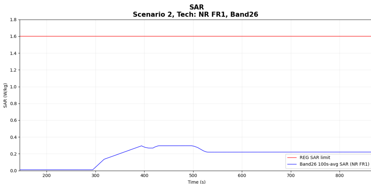
Figure 7-14 Time-averaged SAR
