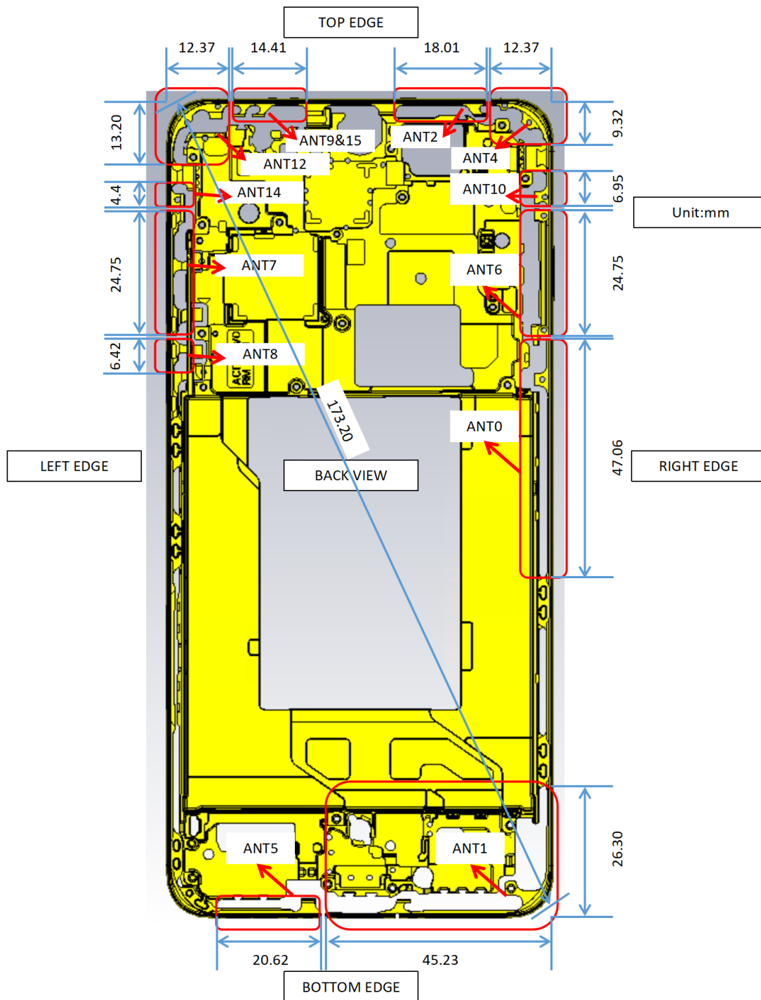
Picture 17: Antenna Locations
