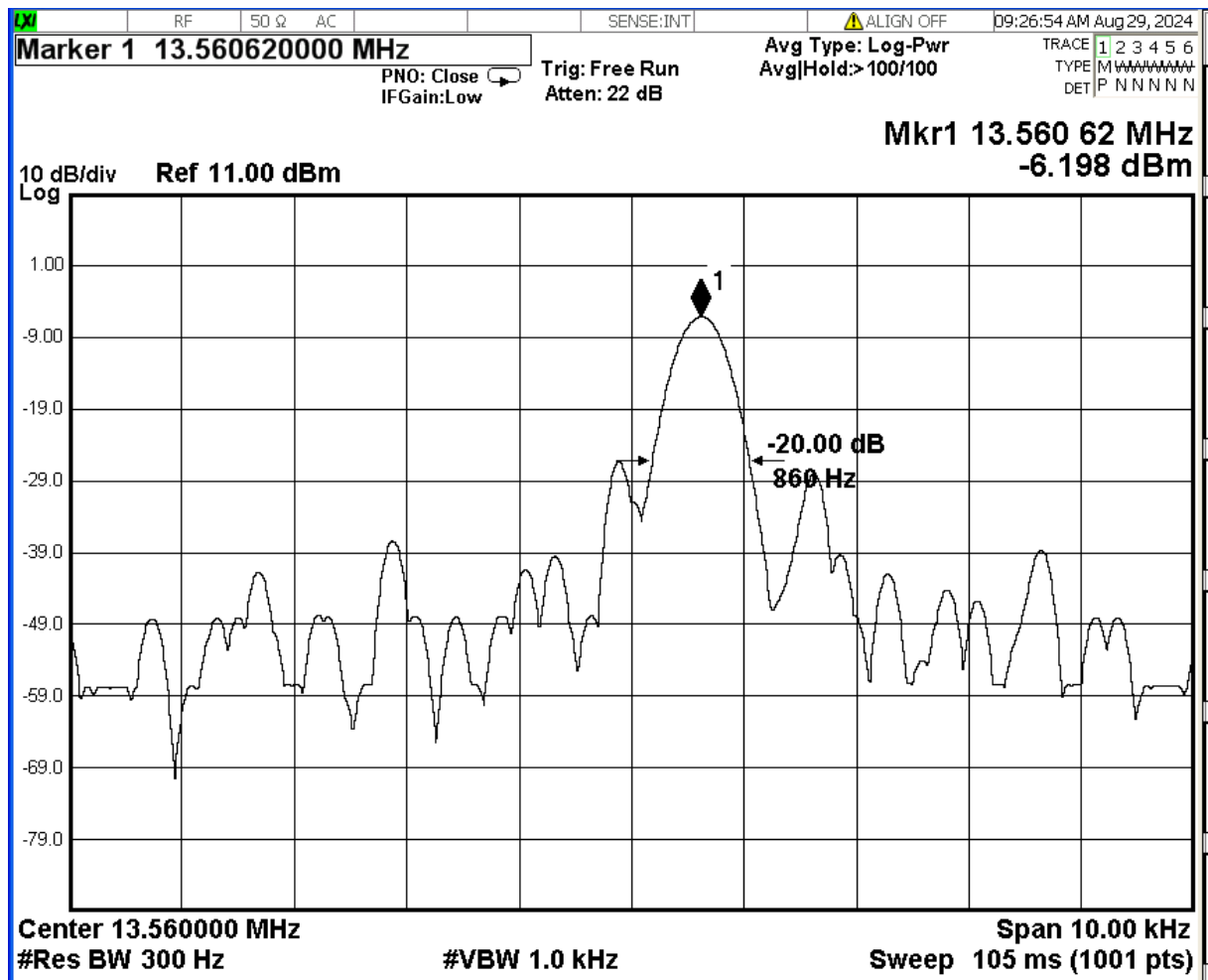
Figure B-9: Measurement results for 20dB Bandwidth
