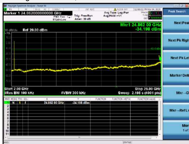
802.11g CHANNEL 9, SPURIOUS 2 GHz ~ 25 GHz
