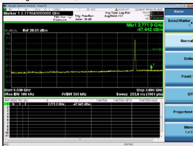
802.11g CHANNEL 9, SPURIOUS 30 MHz ~ 3 GHz
