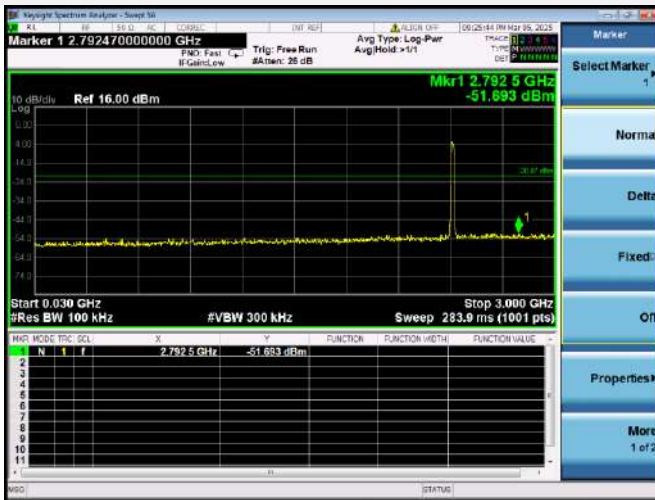
802.11g CHANNEL 2, SPURIOUS 30 MHz ~ 3 GHz
