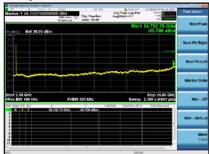
802.11g CHANNEL 3, SPURIOUS 2 GHz ~ 25 GHz
