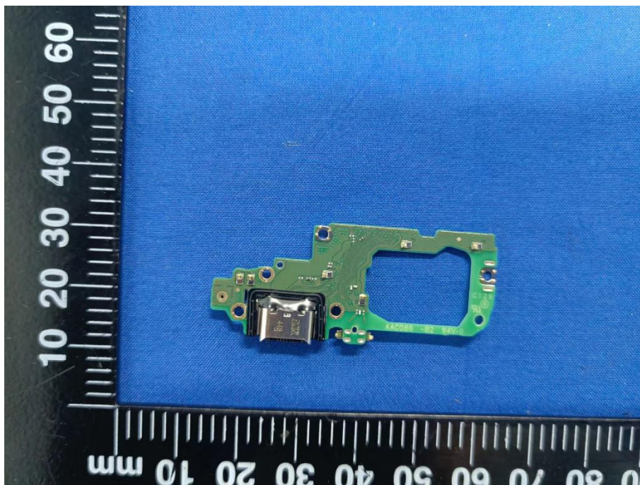
SUB BOARD1 REAR VIEW (WITHOUT SHIELDING)
