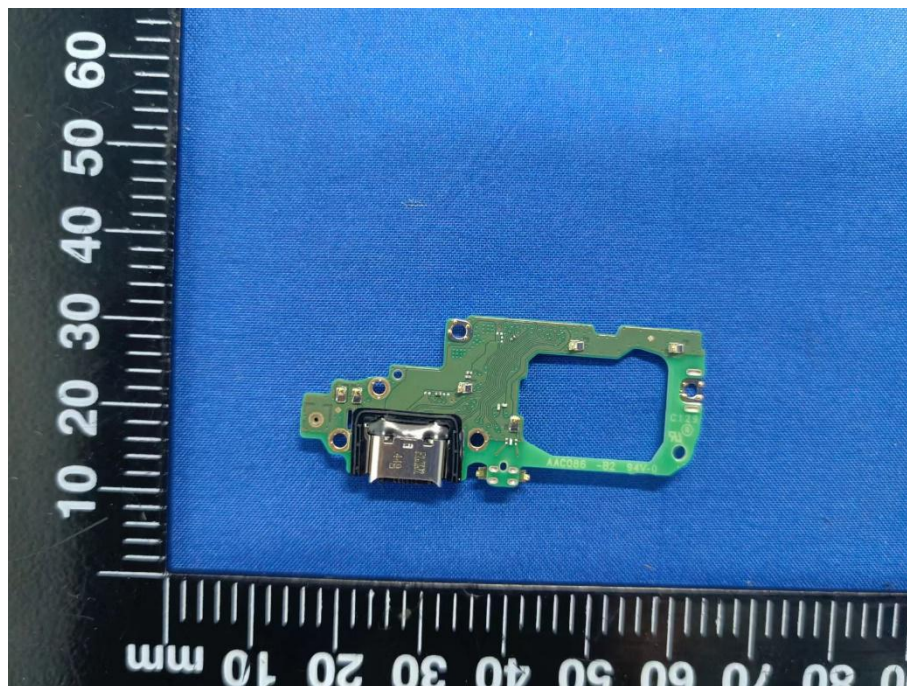
SUB BOARD1 REAR VIEW (WITH SHIELDING)
