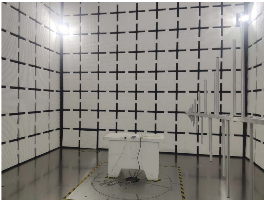
30MHz-1GHz-RF
