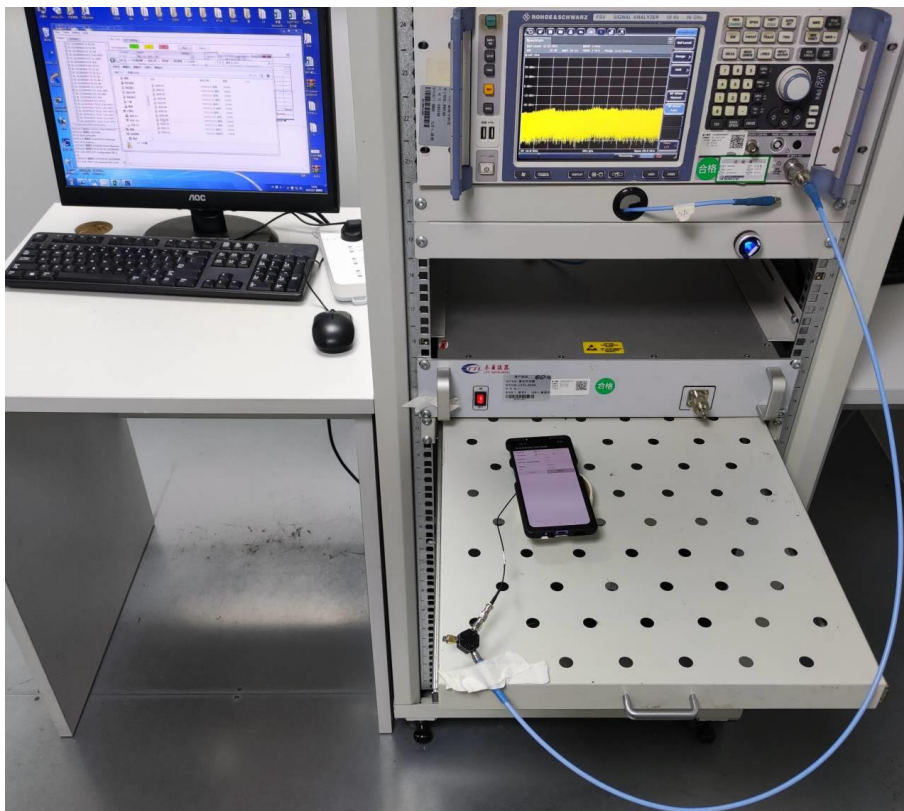
Conducted Test-BLE/WIFI
