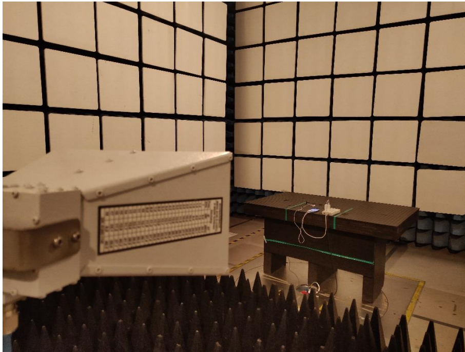
Above 1GHz-RF
