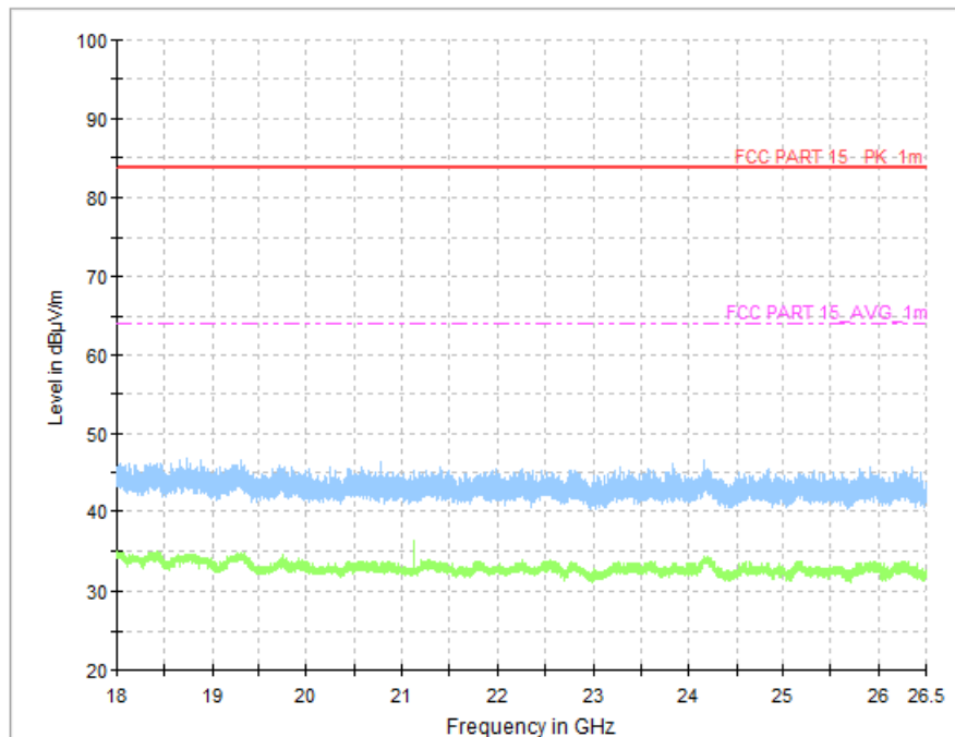
Fig. 59 Radiated Spurious Emission (All Channels, 18GHz ~ 26.5GHz)
