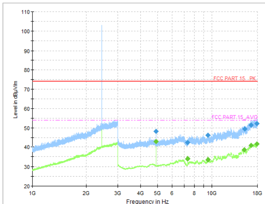
Fig. 43 Radiated Spurious Emission (GFSK, Ch39, 1GHz ~ 18GHz)
