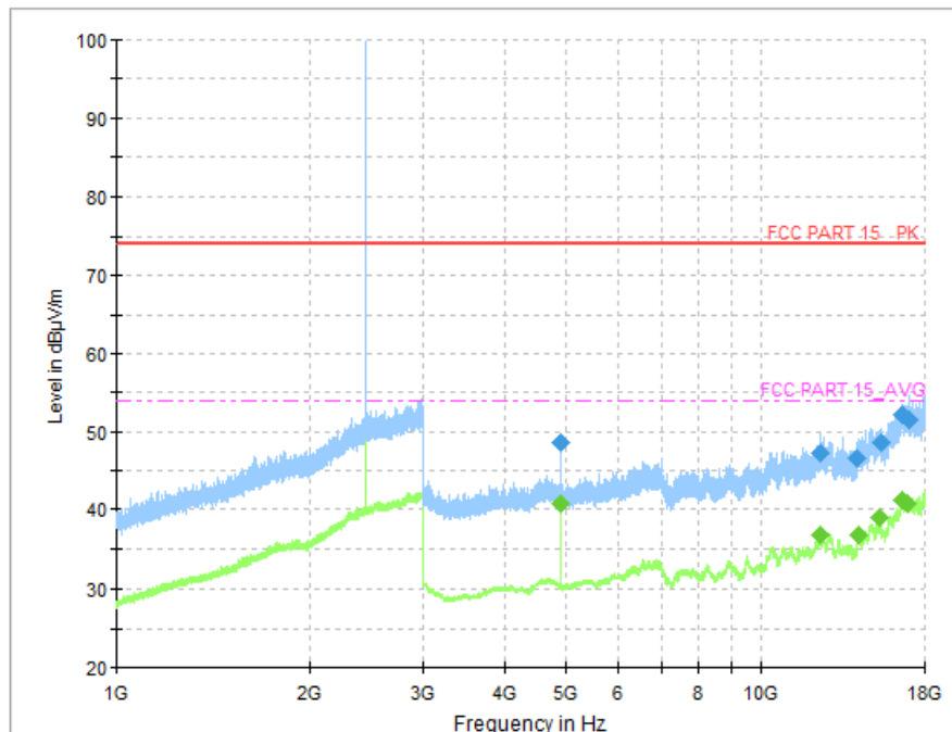
Fig. 53 Radiated Spurious Emission (8DPSK, Ch39, 1GHz ~ 18GHz)
