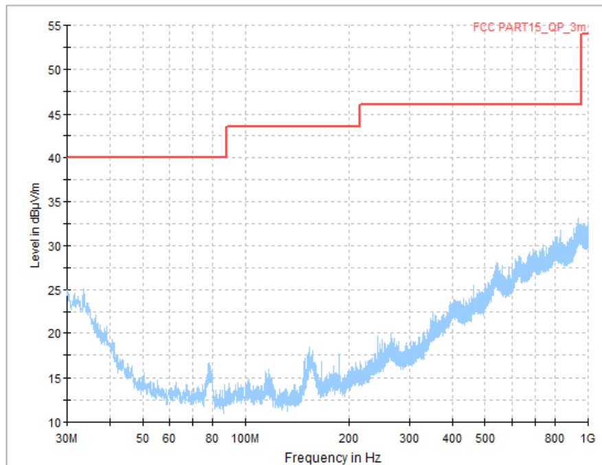
Fig. 58 Radiated Spurious Emission (All Channels, 30MHz ~ 1GHz)
