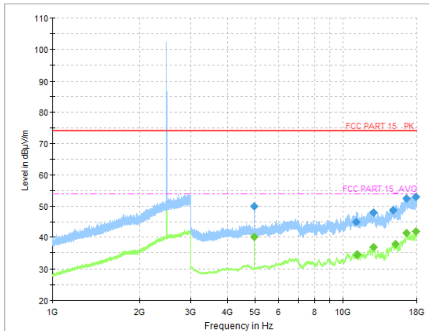
Fig. 54 Radiated Spurious Emission (8DPSK, Ch78, 1GHz ~ 18GHz)
