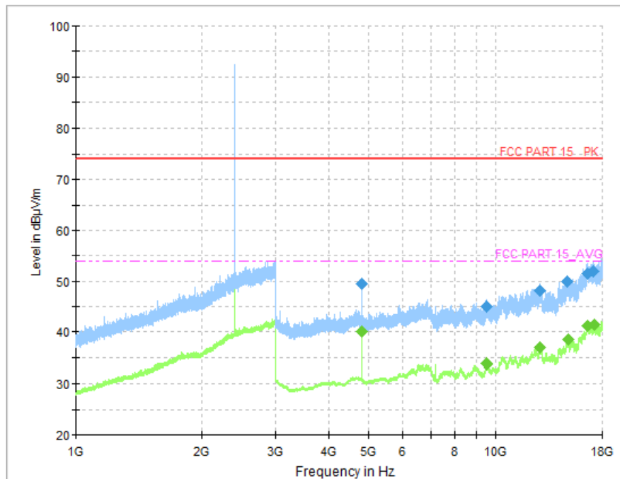
Fig. 52 Radiated Spurious Emission (8DPSK, Ch0, 1GHz ~ 18GHz)
