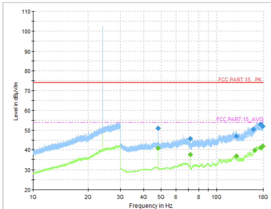
Fig. 42 Radiated Spurious Emission (GFSK, Ch0, 1GHz ~ 18GHz)
