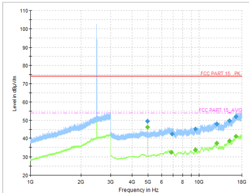
Fig. 44 Radiated Spurious Emission (GFSK, Ch78, 1GHz ~ 18GHz)
