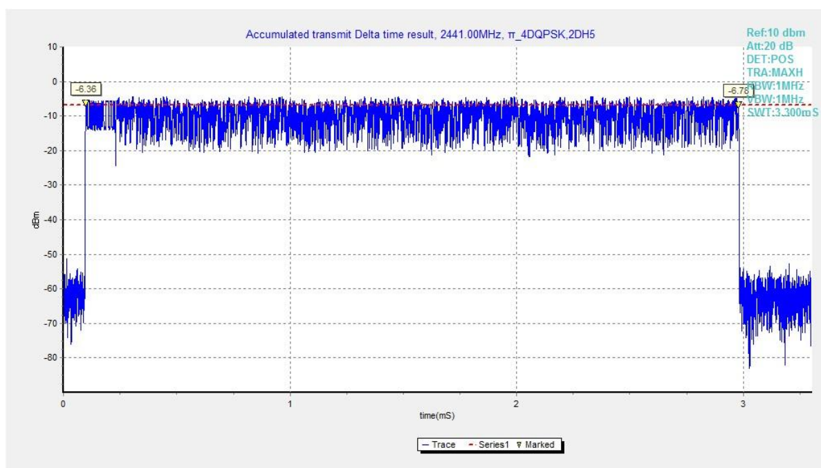
Fig. 71 Time of Occupancy(Dwell Time) ( \pi/4 DQPSK, Ch39)
