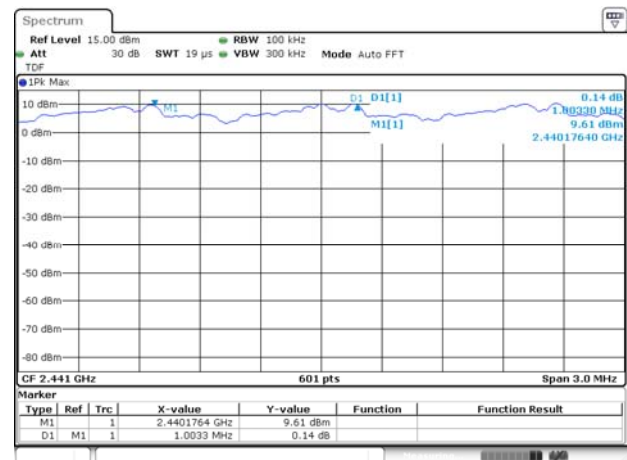
8-DPSK
