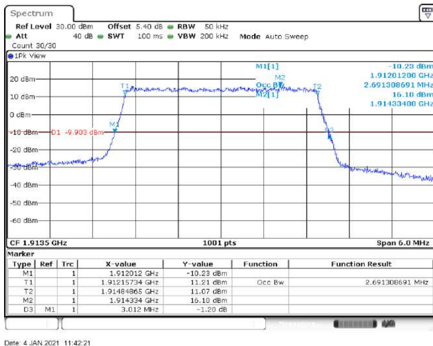
Band25-3MHz-64QAM-26055-15RB#0-2.691
