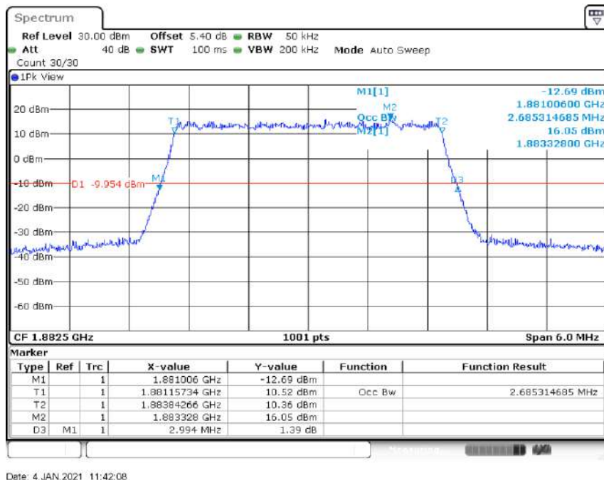
Band25-3MHz-16QAM-26675-15RB#0-2.685
