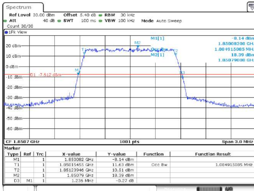
Band25-1.4MHz-QPSK-26047-6RB#0-1.085
