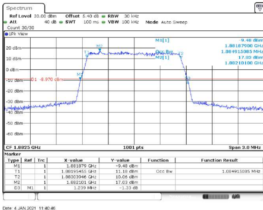
Band25-1.4MHz-16QAM-26683-6RB#0-1.085
