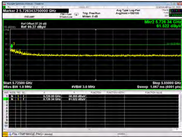
Band III 11ac20 CH140 Peak
