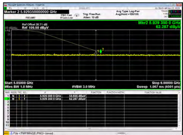
Band IV 11n40 CH159 Peak
