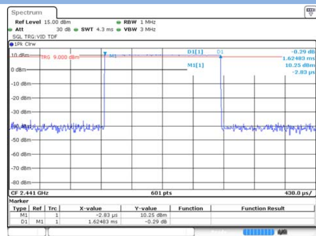
GFSK DH3
