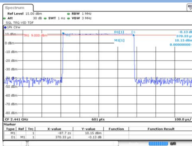
GFSK DH1
