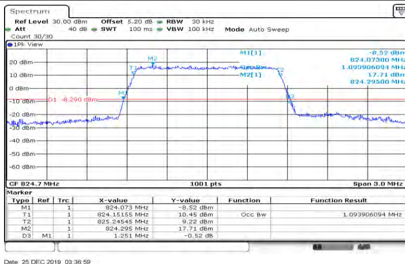
Band26-1.4MHz-16QAM-26915-6RB#0-1.094
