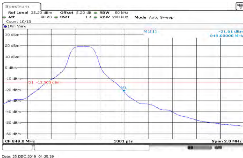
Band 26_5MHz_QPSK_27015_25RB#0
