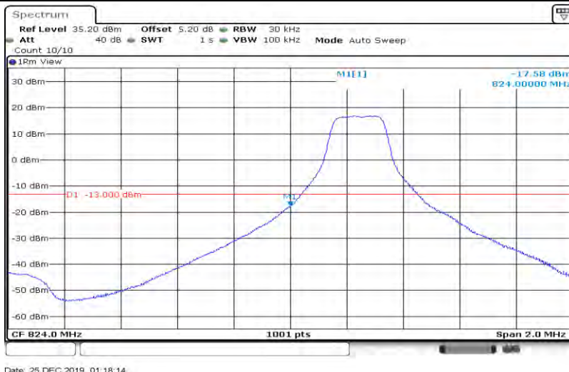
Band 26_3MHz_64QAM_26805_15RB#0
