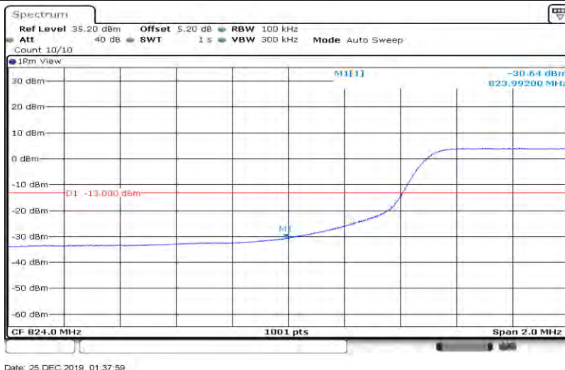
Band 26_10MHz_16QAM_26990_1RB#49
