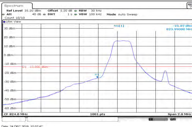
Band 26_1.4MHz_64QAM_26797_6RB#0
