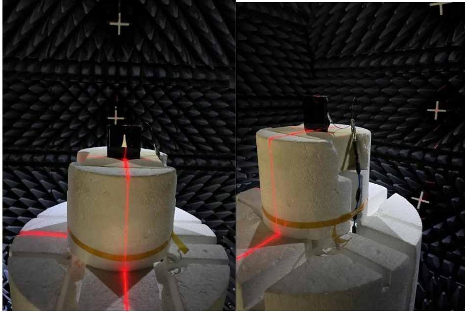
Fig.1. The DUT in the fully anechoic chamber
