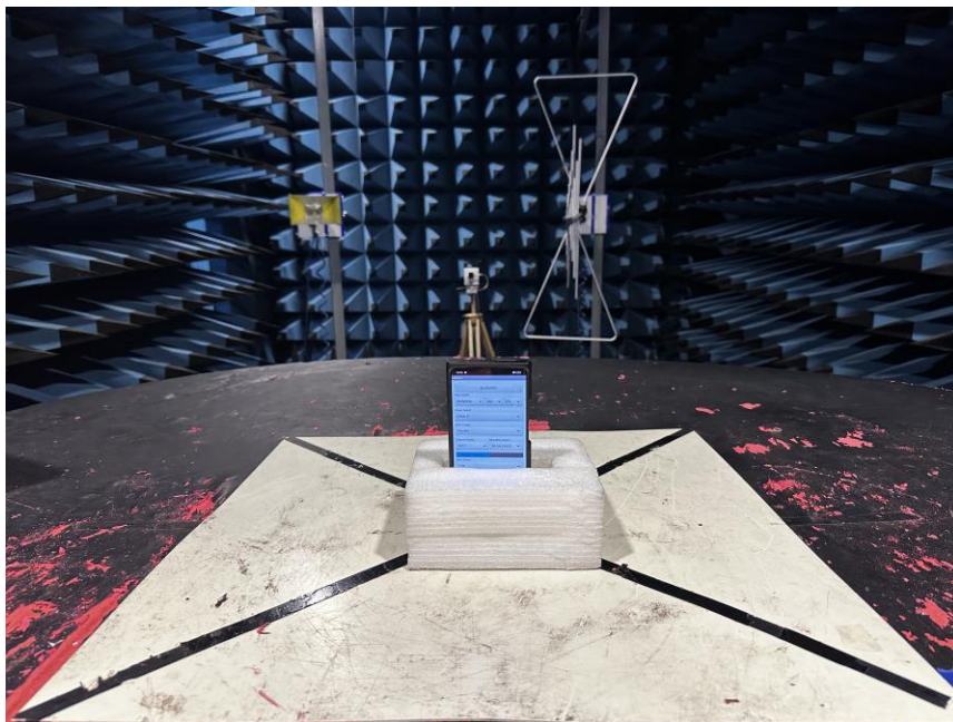
Radiated Emission 18GHz-40GHz
