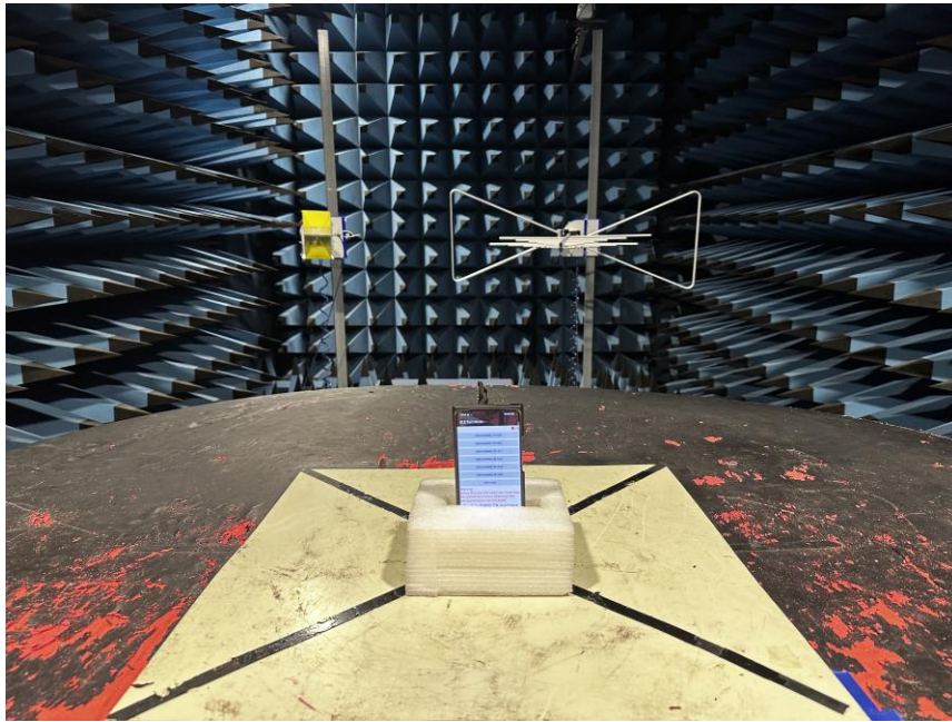
Radiated Emission 1GHz-18GHz
