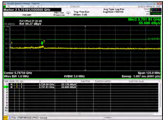
Band III 11a CH140 Peak
