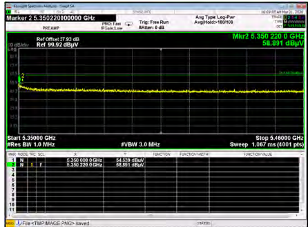
Band II 11n20 CH64 Peak
