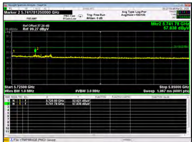
Band III 11n40 CH134 Peak
