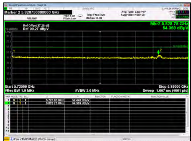
Band III 11ac40 CH134 Peak
