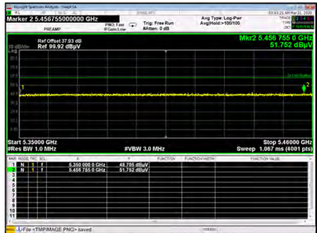
Band II 11ac20 CH64 Peak
