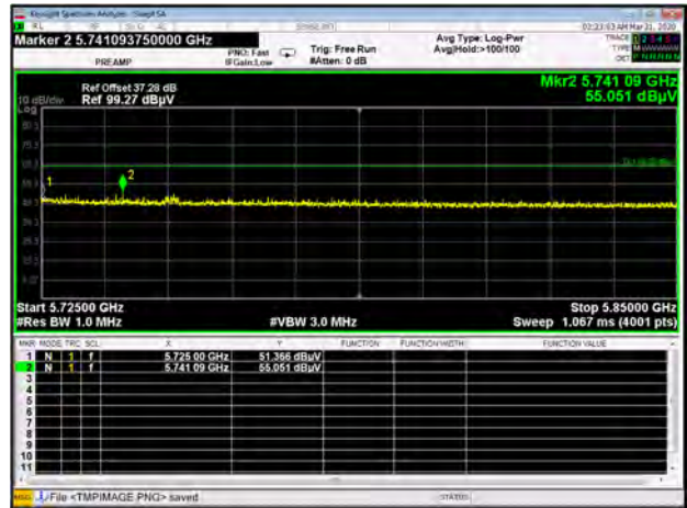
Band III 11n20 CH140 Peak
