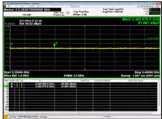
Band II 11a CH64 Peak
