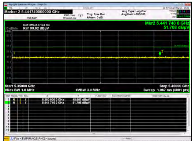
Band II 11n20 CH64 Peak
