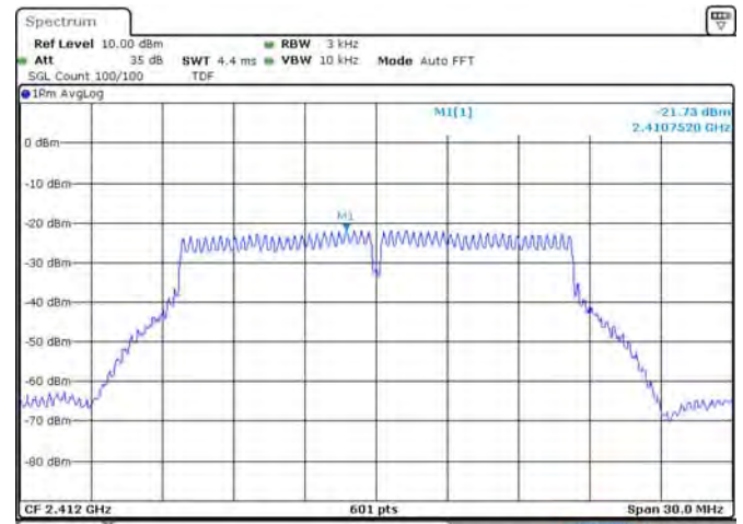
802.11g LOW CHANNEL
