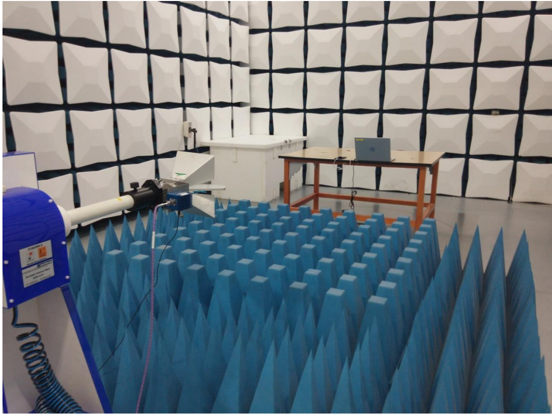
FCC Part15B Radiated Emission 1GHz-18GHz
