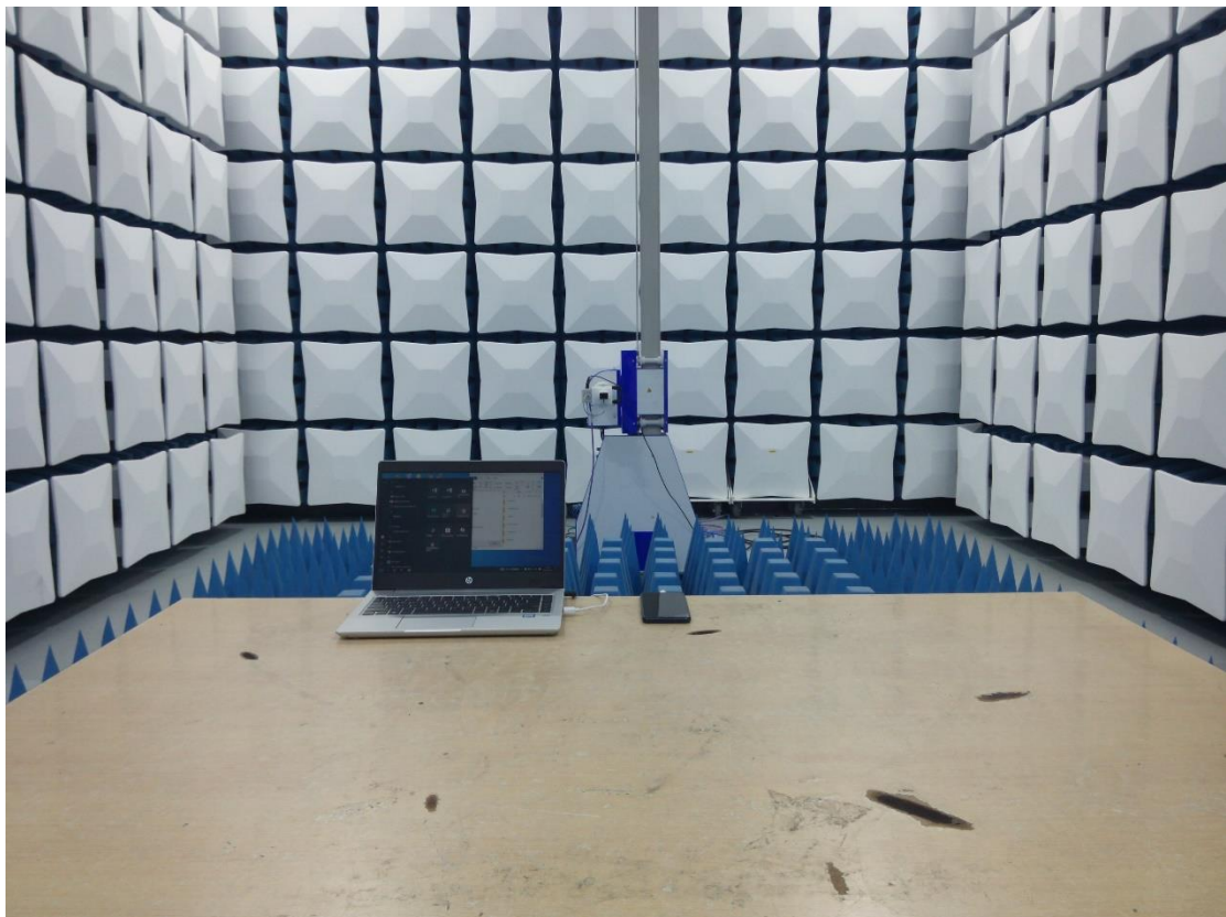
FCC Part15B Radiated Emission 18GHz-26.5GHz
