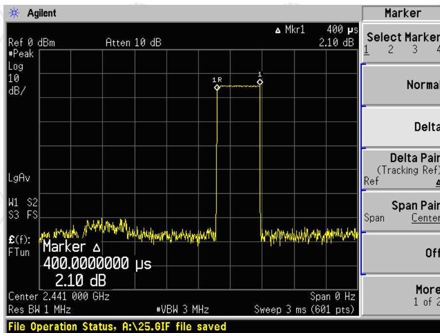
2441 MHz_DH1
