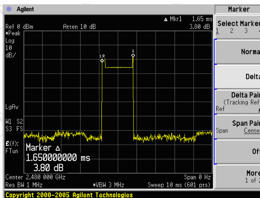
2480 MHz_DH3
