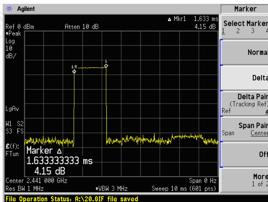
2441 MHz_DH3
