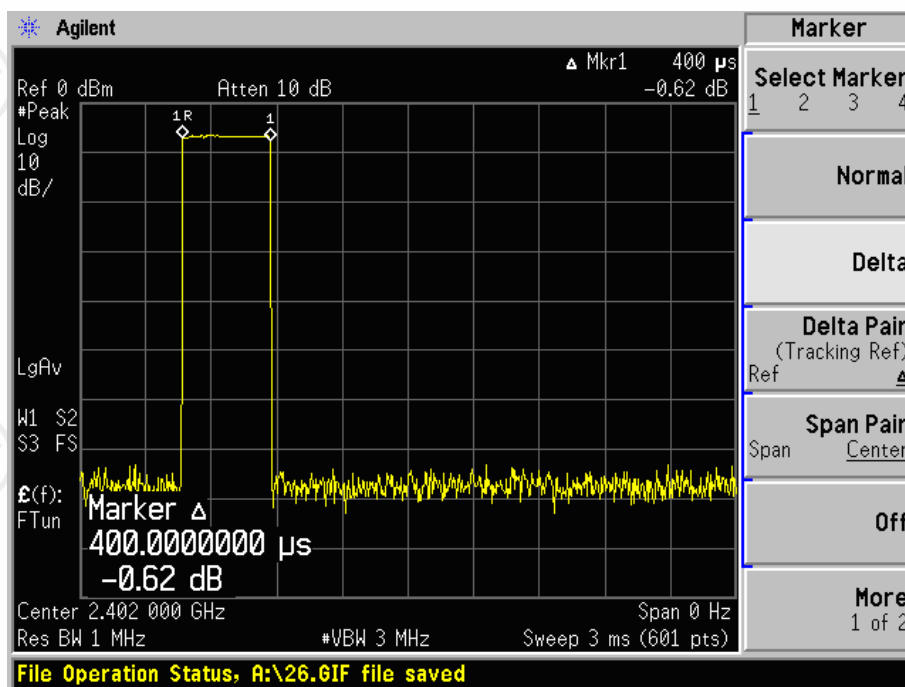
2402 MHz_DH1
