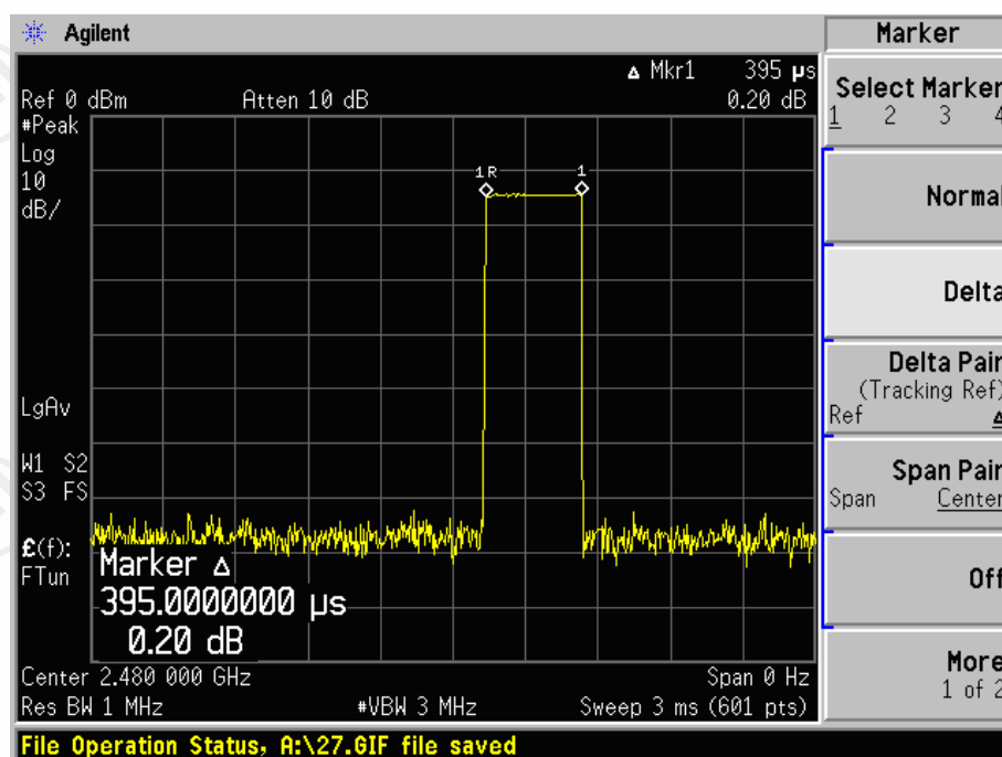
2480 MHz_DH1
