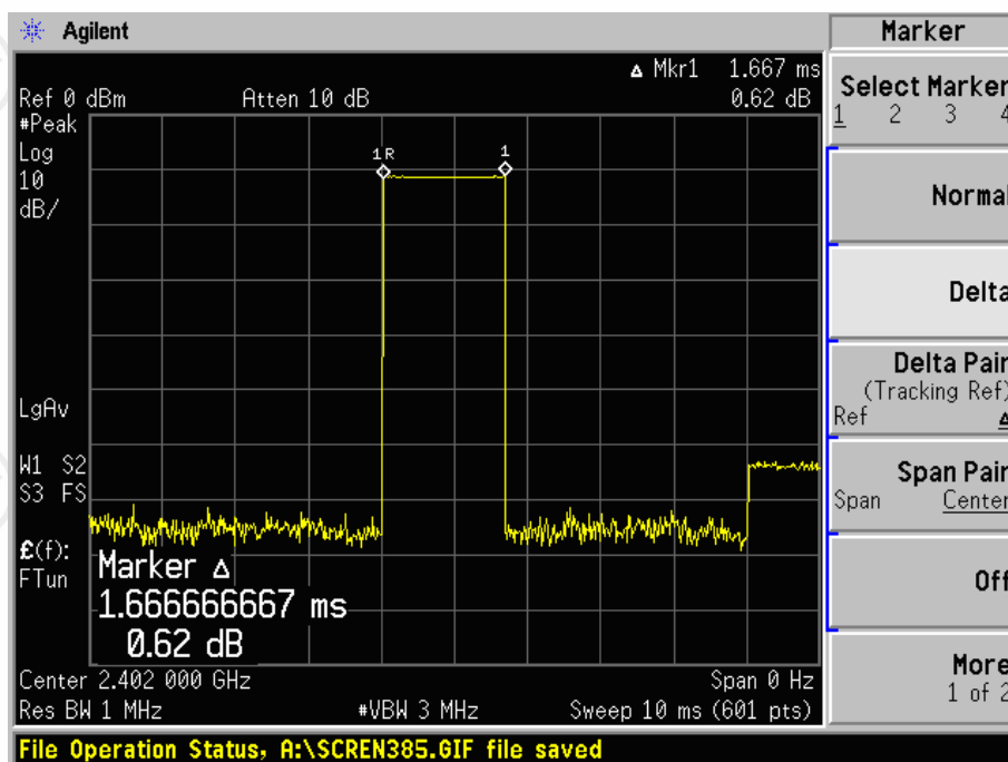
2402 MHz_DH3
