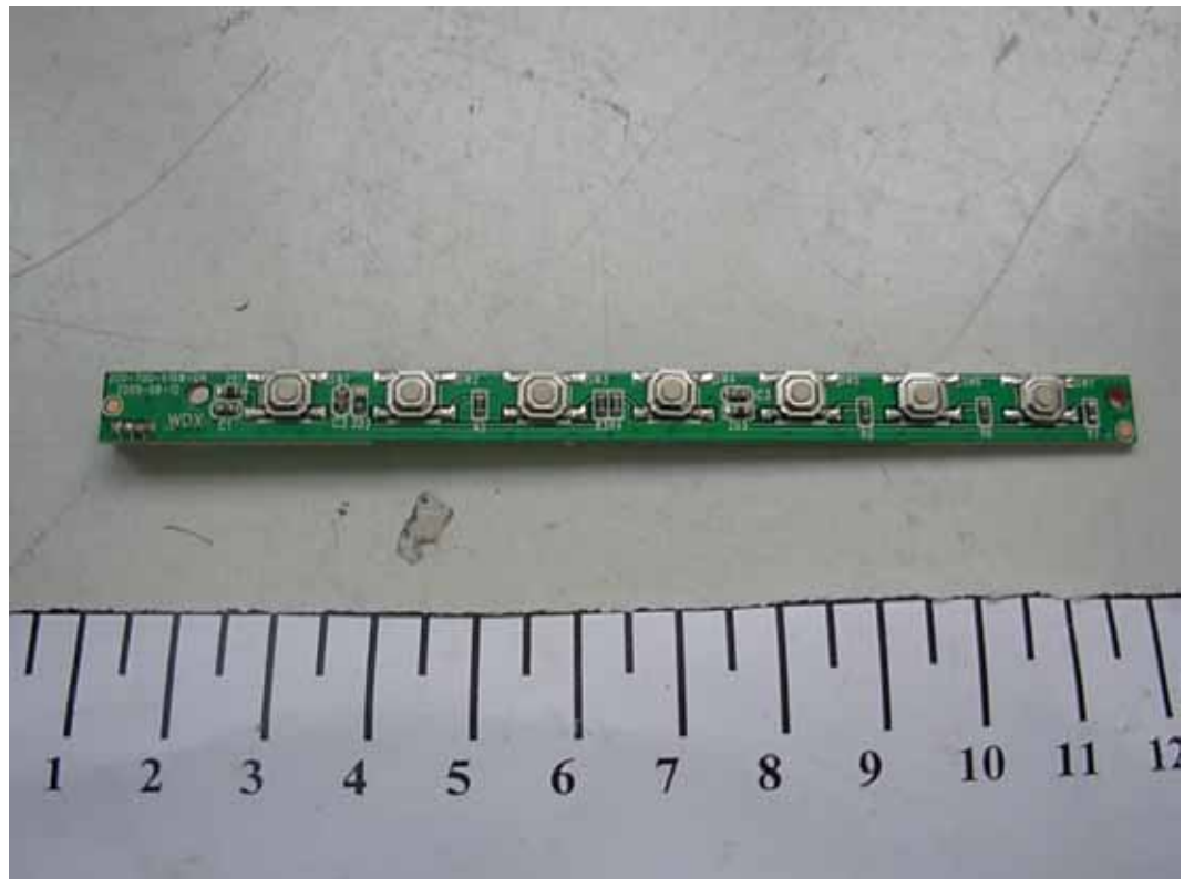
FIGURE 6 LCD TV (M/N: ELETT221) KEY BOARD (COMPONENT SIDE)
