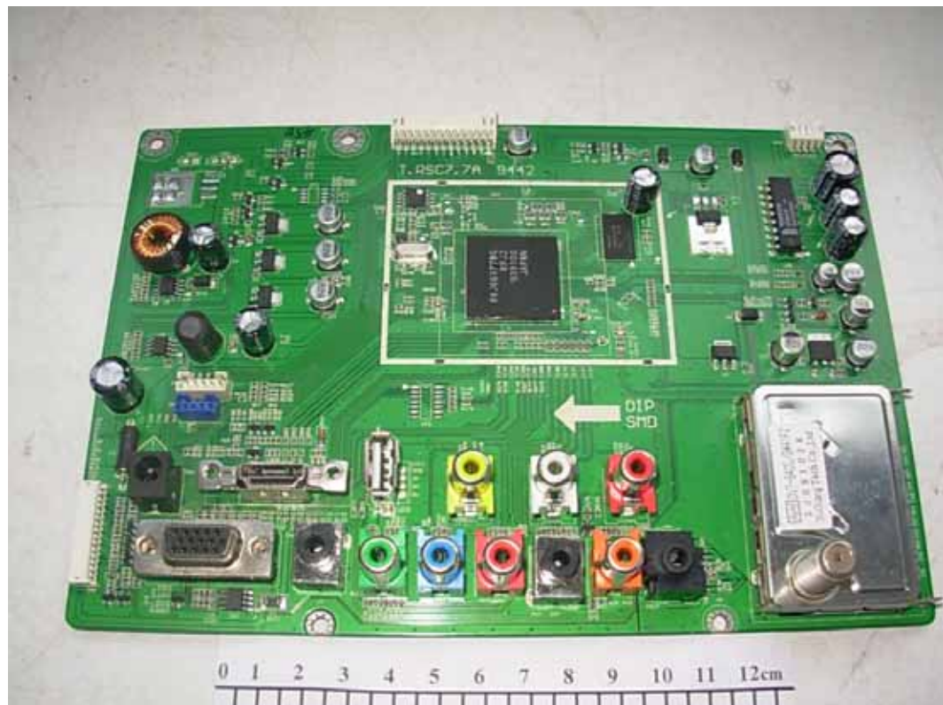
FIGURE 2 LCD TV (M/N: ELETT221) MAIN BOARD (COMPONENT SIDE)
