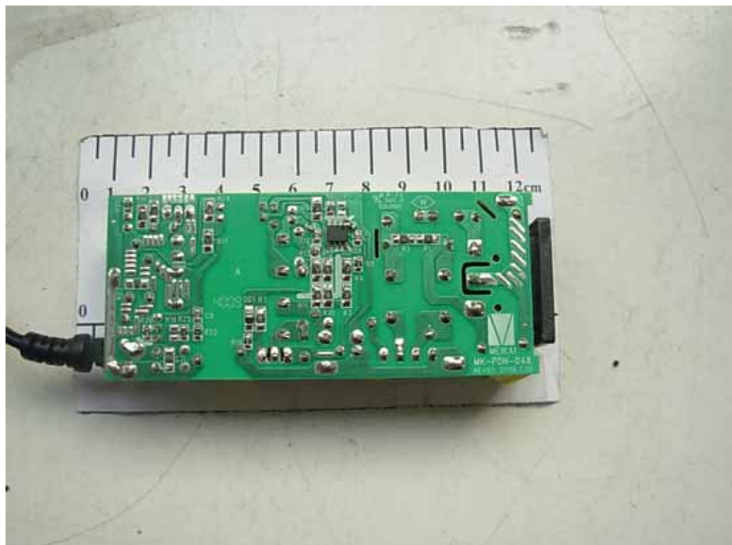
FIGURE 9 LCD TV (M/N: ELETT221) ADAPTER (POWER BOARD – SOLDERED SIDE)
