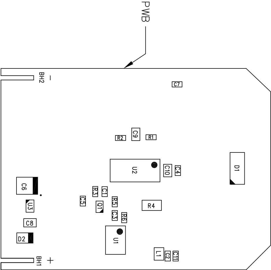
VIEW FROM BOTTOM SIDE BOTTOM ASSEMBLY
