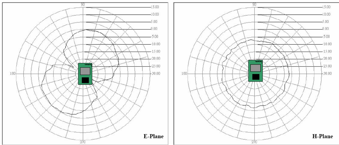
Figure 6. Module in vertical antenna pattern
