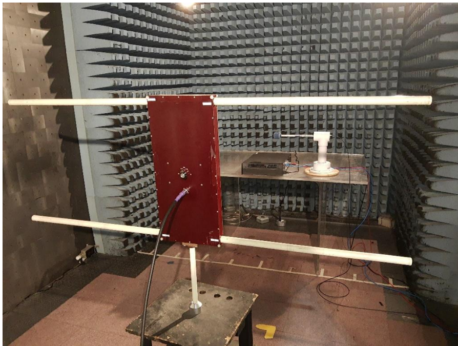
Figure 2: Radiated Immunity - Test Setup for 1MHz
