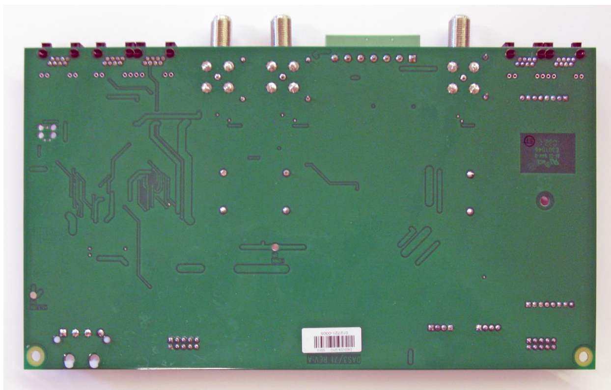
GPIO and Radio Module underside
