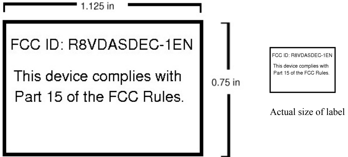
Drawing of DASDEC FCC Label
