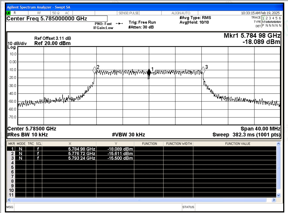
Freq. Stability NVNT a 5785MHz Ant4
