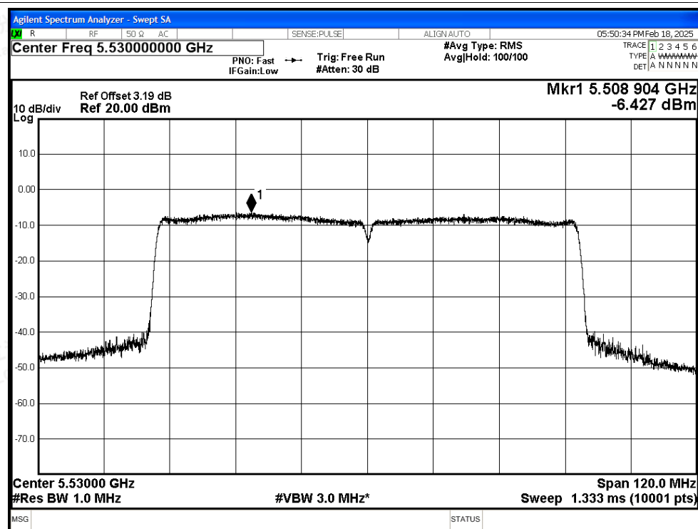
PSD NVNT ac80 5530MHz Ant3
