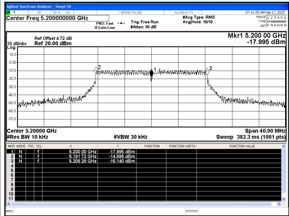
Freq. Stability NVNT a 5200MHz Ant4
