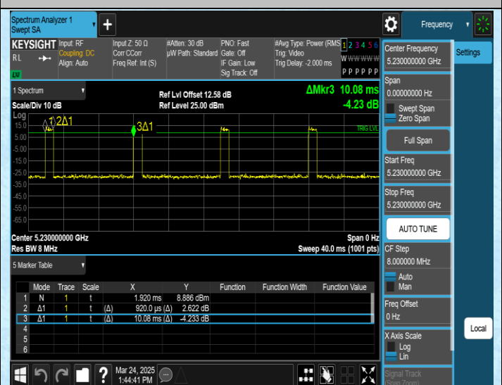
NTNV-11AC40SISO-Ant2-5230
