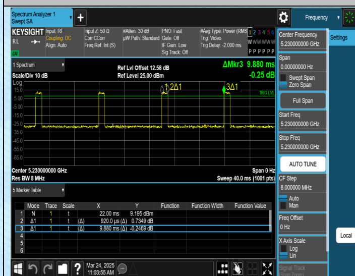
NTNV-11AC40SISO-Ant1-5230
