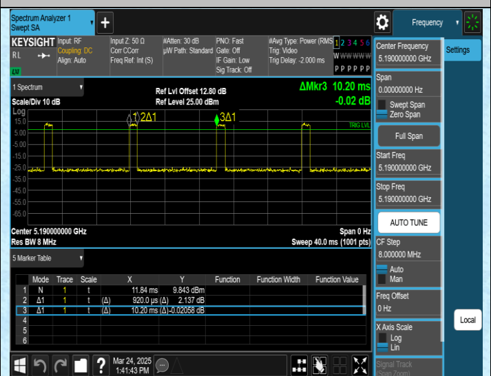
NTNV-11AC40SISO-Ant2-5190
