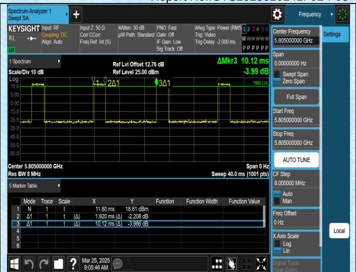
NTNV-11AC20SISO-Ant2-5805
