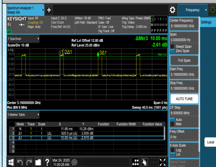
NTNV-11AC40SISO-Ant1-5190
