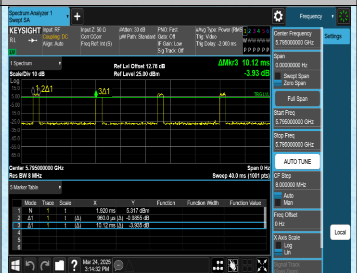
NTNV-11AC40MIMO-Ant2-5795
