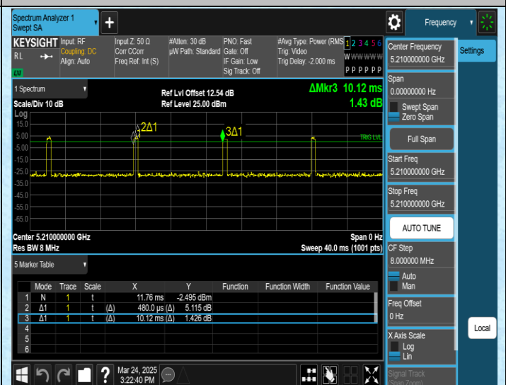
NTNV-11AC80MIMO-Ant2-5210
