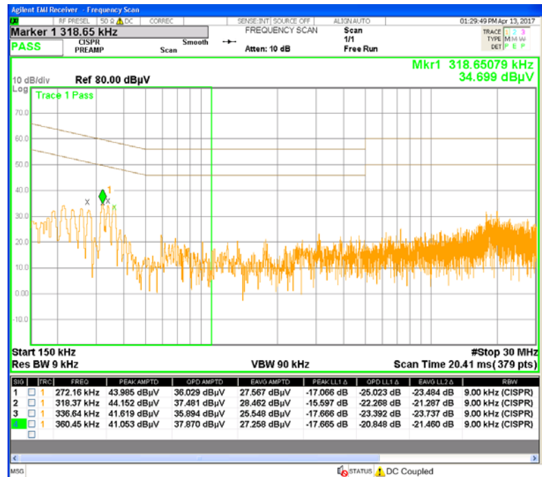
Plot # 73. AC line conducted emissions test. Line Neutral.
