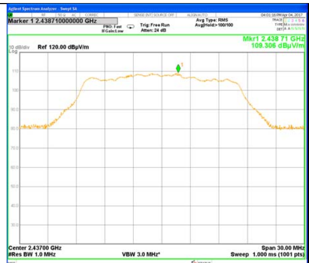
Plot # 17. Carrier frequency – 2437 MHz
