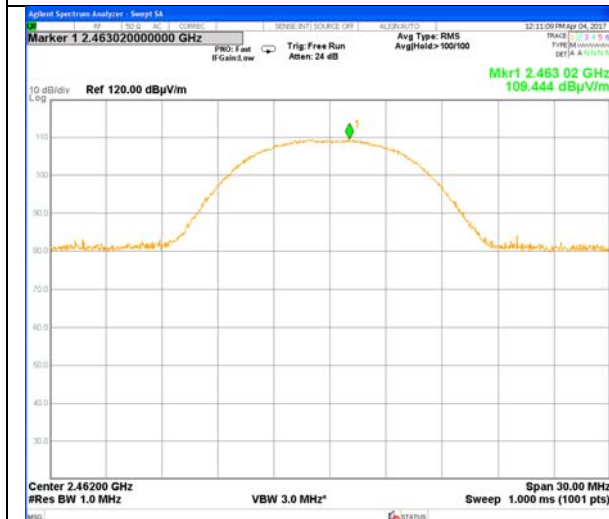
Plot # 15. Carrier frequency – 2462 MHz
